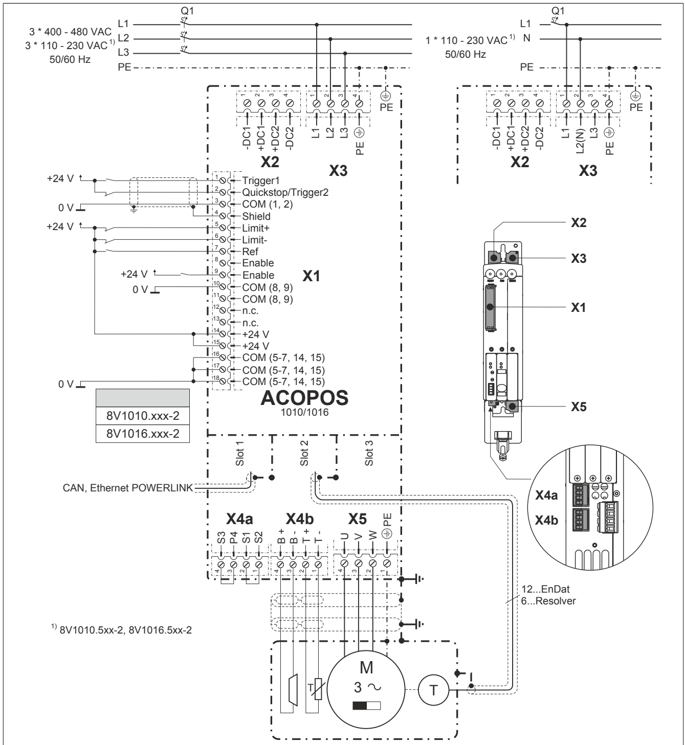
Figure 13: ACOPOS 1010, 1016 - Pinout overview
