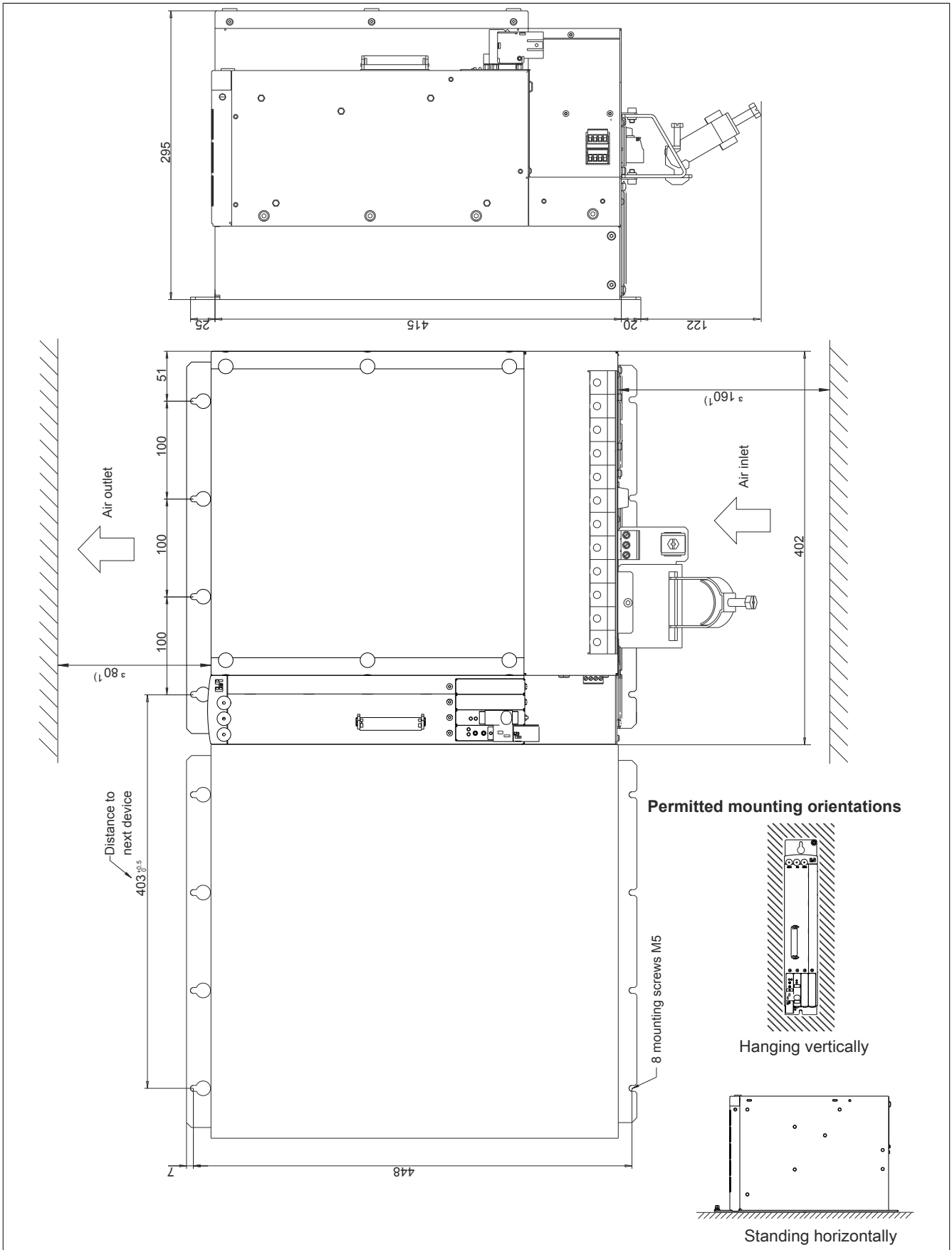
Figure 58: ACOPOS 128M - Dimension diagram and installation dimensions
