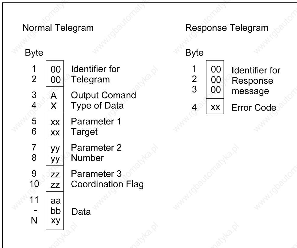
Fig. 4-7: Structure of an output telegram from 3964 (R) with RK512
