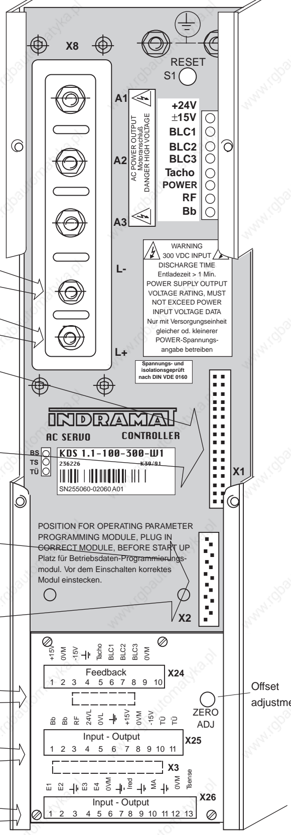
Figure 40: Front view of servo drive module KDS1 with accessories
