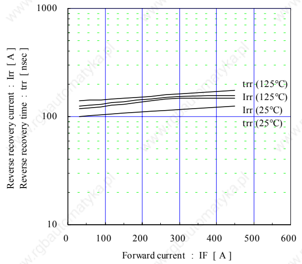
Reverse recovery characteristics (typ.) V_{ce}=V, V_{GE}=\pm 15\text{V}, R_g=2\Omega
