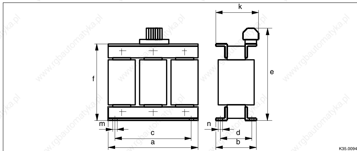
FIG 13-5 Mains chokes with connection lug
