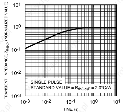
TRANSIENT THERMAL IMPEDANCE CHARACTERISTICS (Each FWDt)
