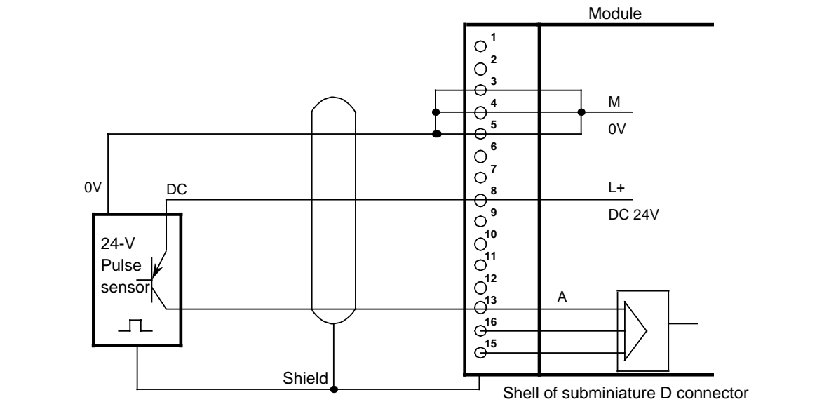
Figure 15-10. Connecting a Counting Pulse Sensor for 24 V DC
