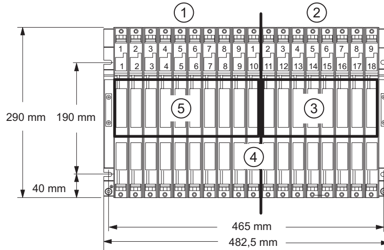
Figure 2-4 CR2 rack
