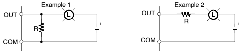
Generating a dark current (about 1/3 of the rated current) through the incandescent bulb.
