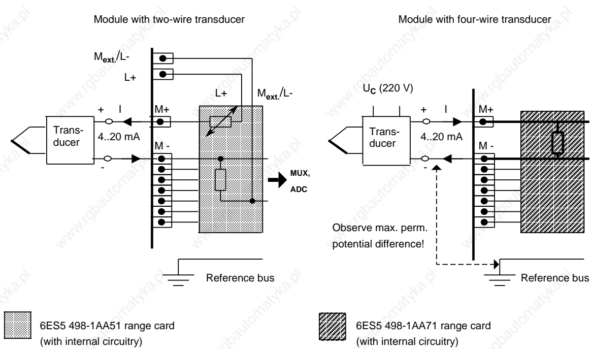
Figure 10-8. Connecting Transducers
