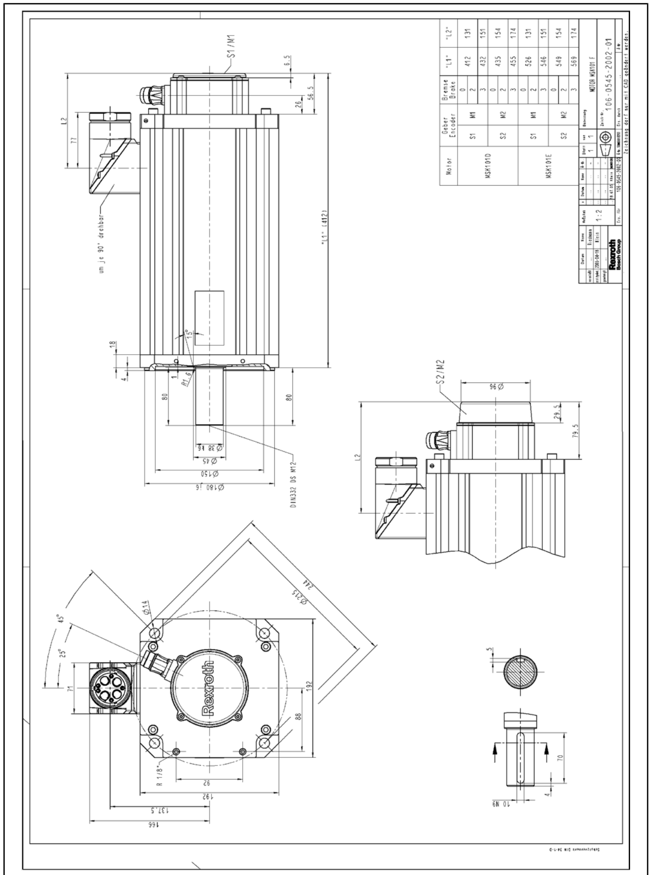
Fig.5-14: MSK101...FN specification
