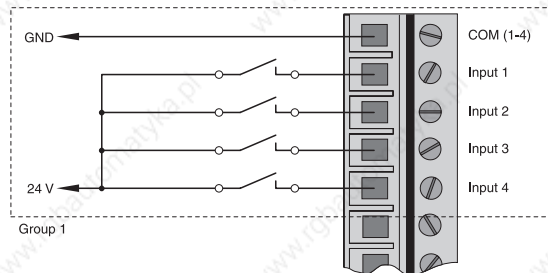
Sink Circuit:
