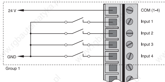
Source Circuit:
