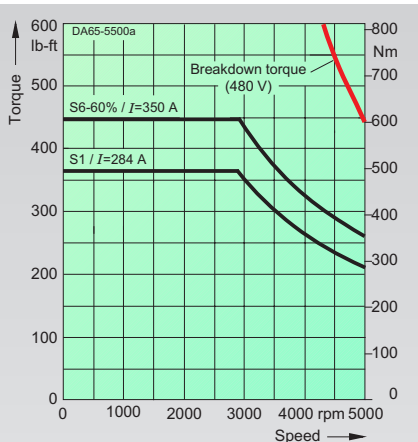
1PL6186-4.L. max. breakdown torque: 1330 lb-ft/1803 Nm
