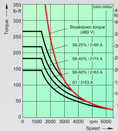
1PH7163-2.D...-.... max. breakdown torque: 538 lb-ft/730 Nm
