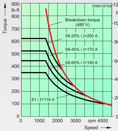
1PH7186-2.D...-.... max. breakdown torque: 858 lb-ft/1163 Nm
