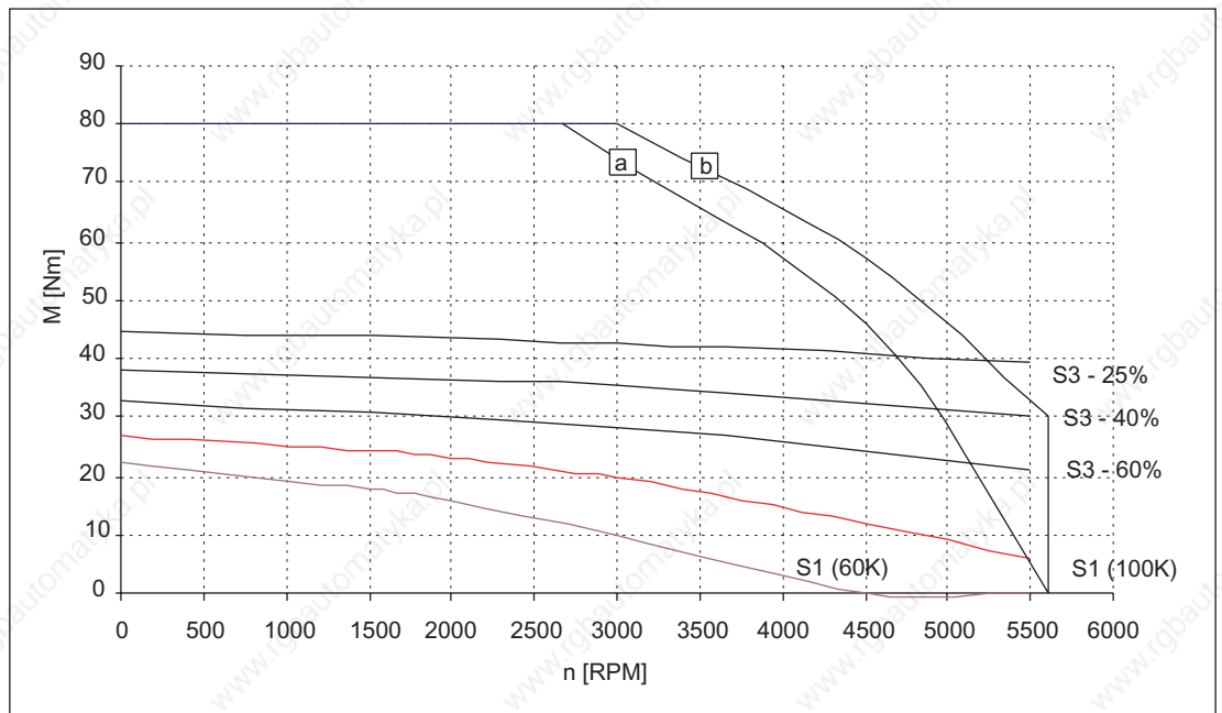
Figure 3-39 Speed-torque diagram 1FT6102-8AH7□
