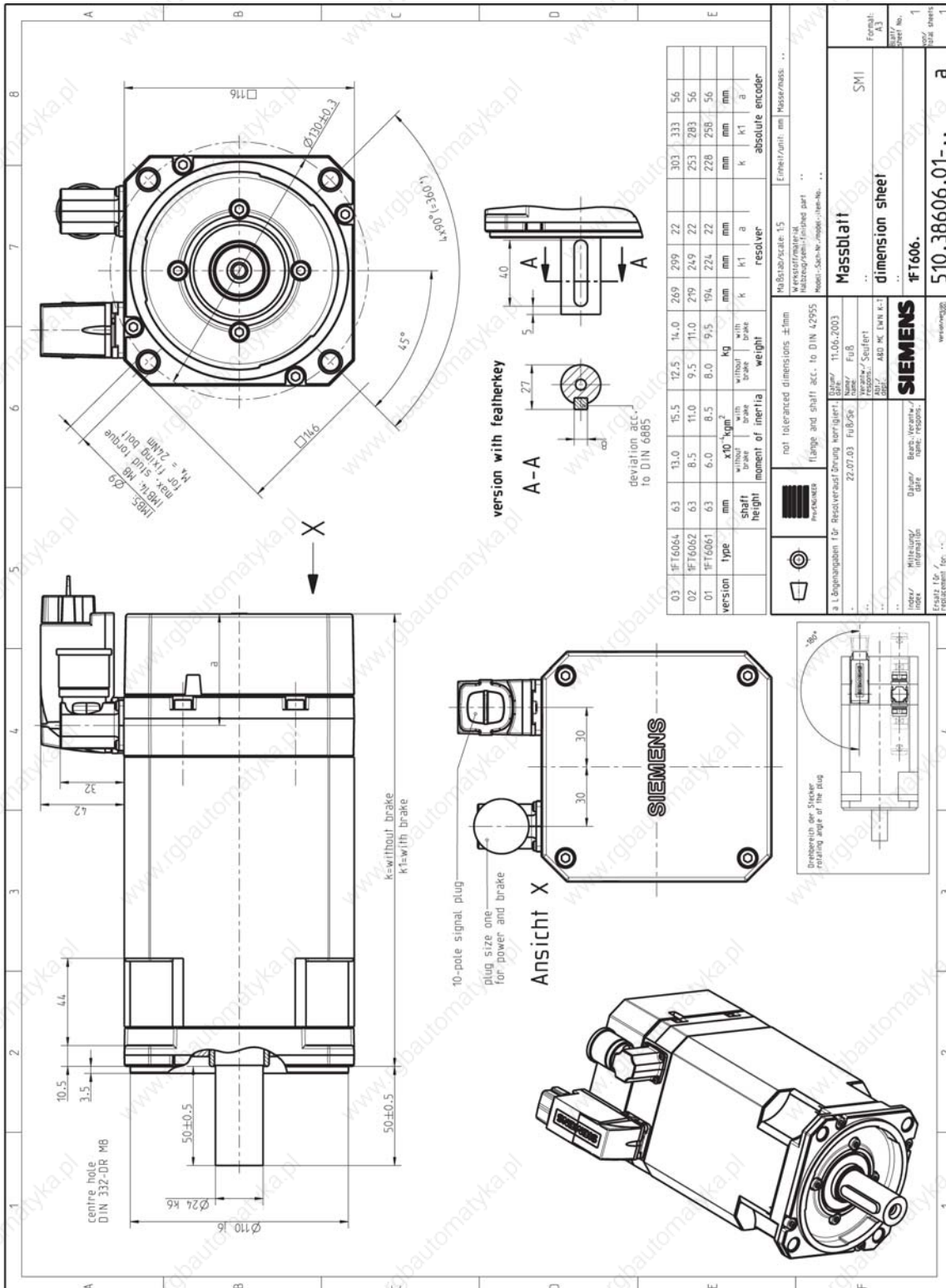
Figure 5-4 1FT606□-□A□DQ
