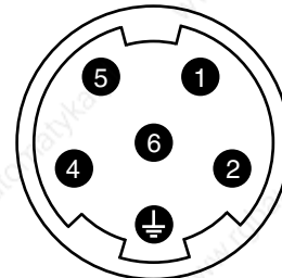
INTERCONNECTRON SIZE 1 6 PIN
