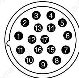
INTERCONNECTRON SIZE 1 17 PIN
