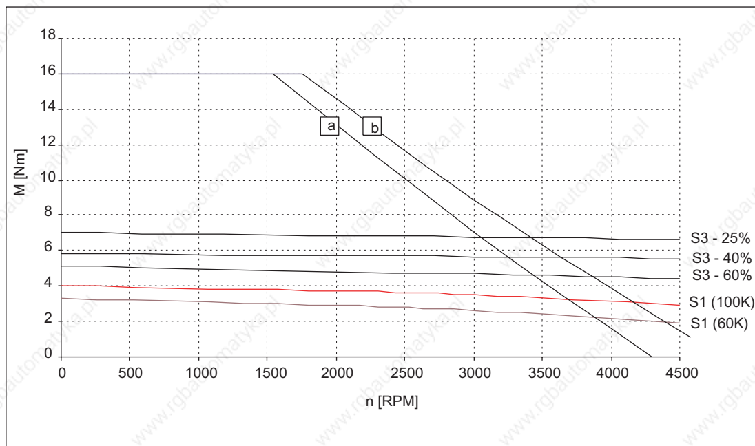
Figure 3-10 Speed-torque diagram 1FT6061-6AF7□
