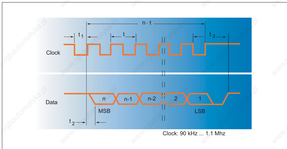
Figure 4-3 Output signals, absolute value encoders
