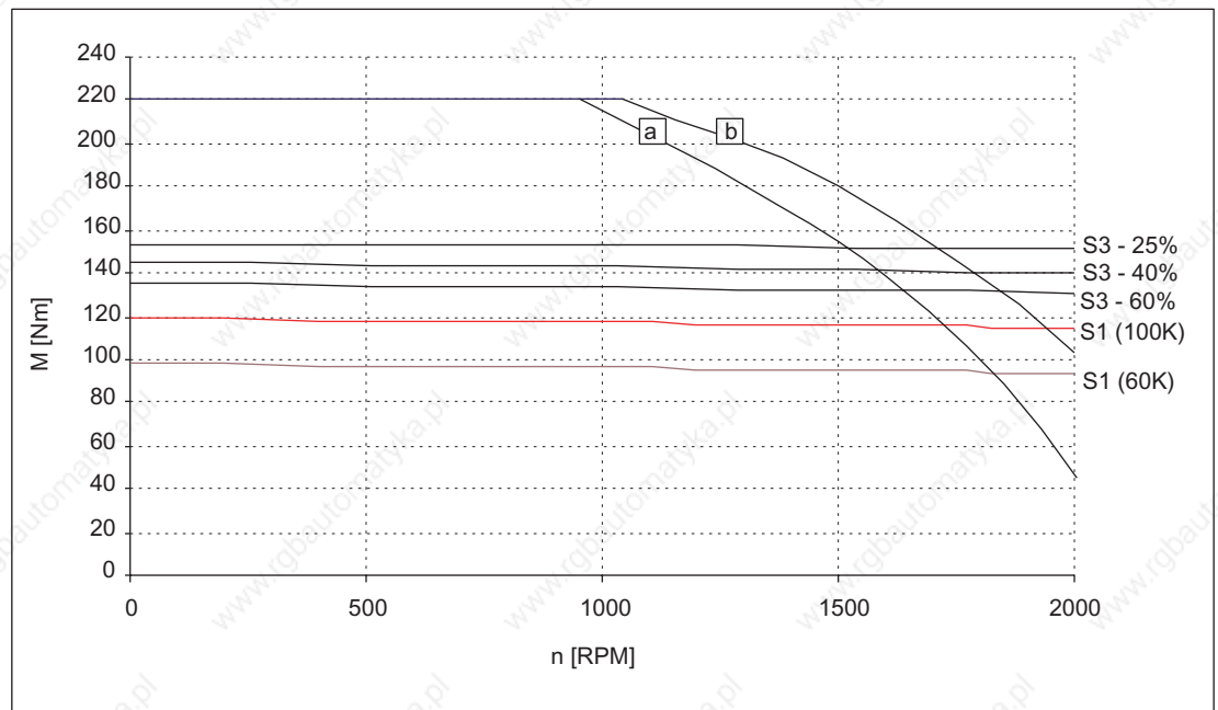
Figure 3-92 Speed-torque diagram 1FT6108-8WB7□
