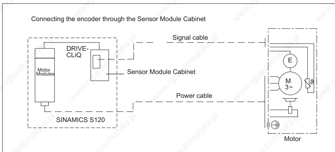
Figure 2-5 Connecting encoders without DRIVE-CLiQ
