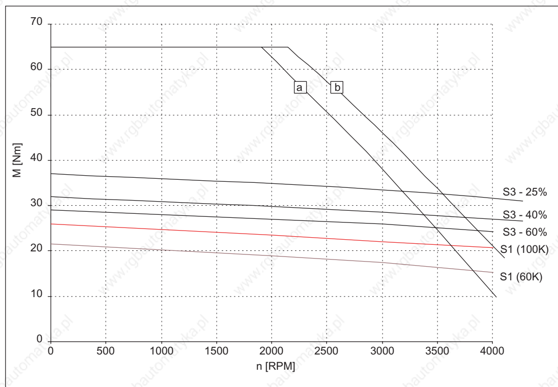
Figure 3-53 Speed-torque diagram 1FT6084-8SF7
