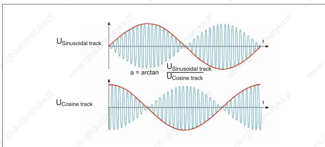
Figure 4-4 Output signals, resolver
