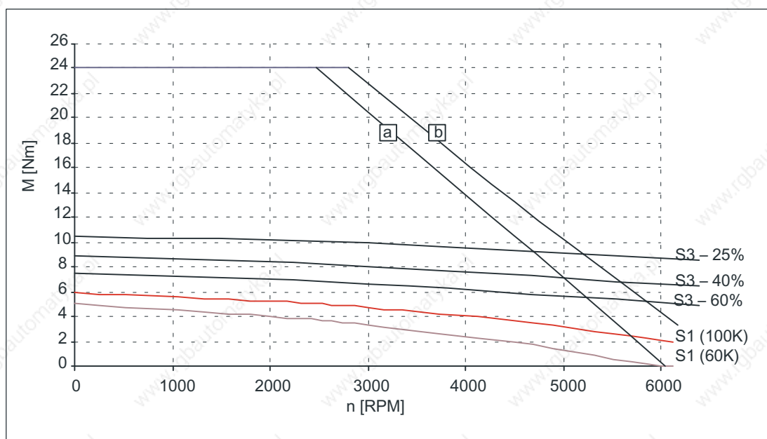
Figure 3-15 Speed-torque diagram 1FT6062-6AH7□
