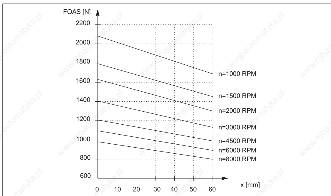
Figure 3-111 Cantilever force F_Q at a distance x from the shaft shoulder for a nominal bearing lifetime of 20,000 h
