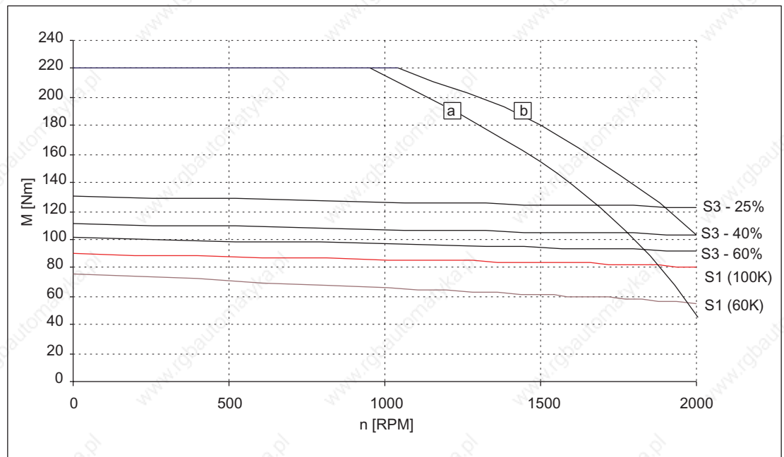
Figure 3-63 Speed-torque diagram 1FT6108-8SB7□
