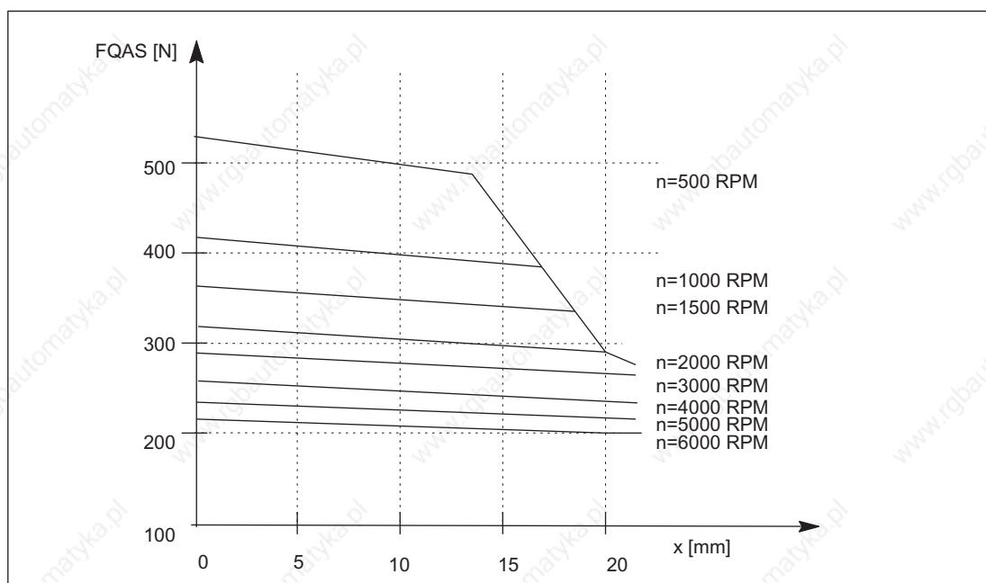
Figure 3-107 Cantilever force F_Q at a distance x from the shaft shoulder for a nominal bearing lifetime of 20,000 h
