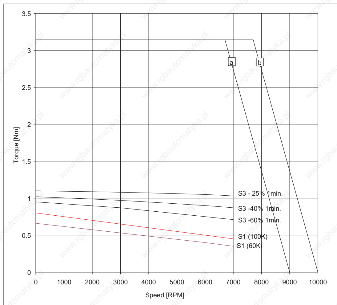
Figure 3-2 Speed-torque diagram 1FT6024-6AK71
