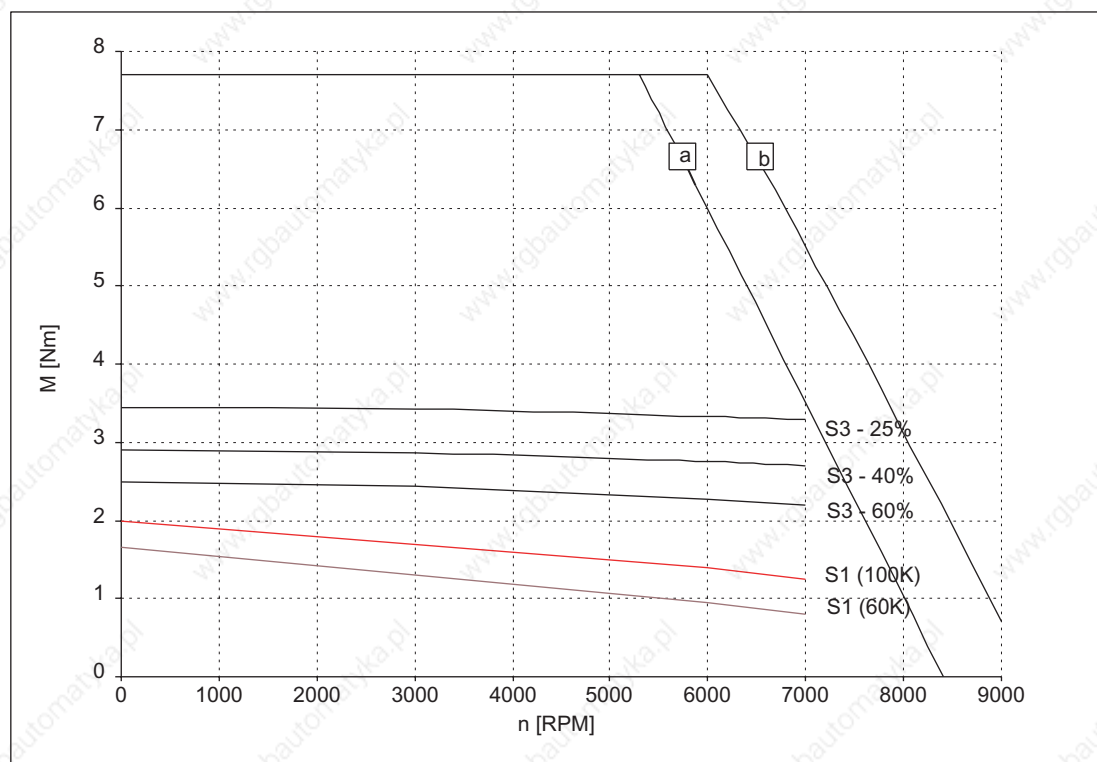
Figure 3-4 Speed-torque diagram 1FT6034
