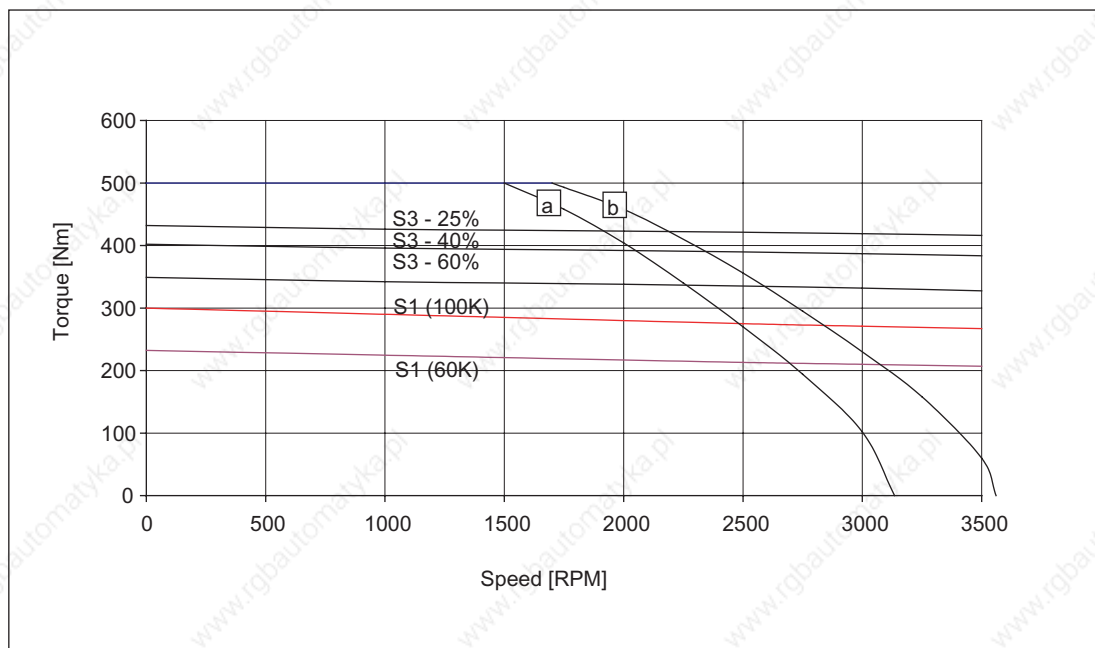
Figure 3-102 Speed-torque diagram 1FT6138-6WD7□
