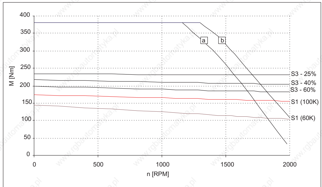
Figure 3-72 Speed-torque diagram 1FT6136-6SB71
