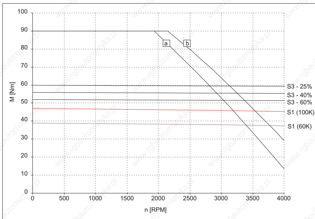
Figure 3-87 Speed-torque diagram 1FT6086-8WF7
