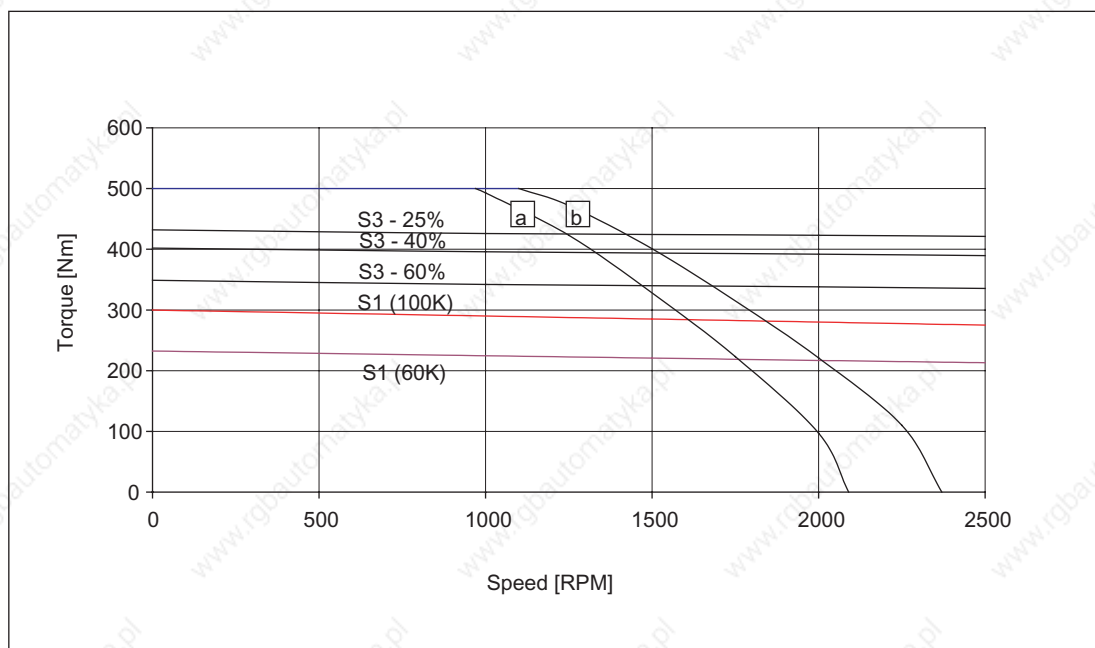
Figure 3-101 Speed-torque diagram 1FT6138-6WB7□
