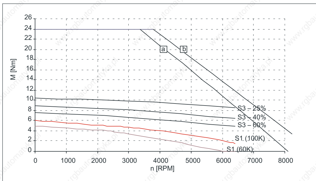
Figure 3-16 Speed-torque diagram 1FT6062-6AK7□
