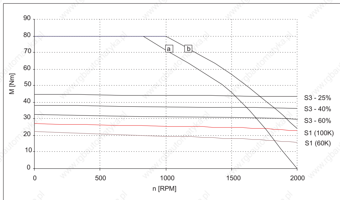
Figure 3-36 Speed-torque diagram 1FT6102-8AB7□
