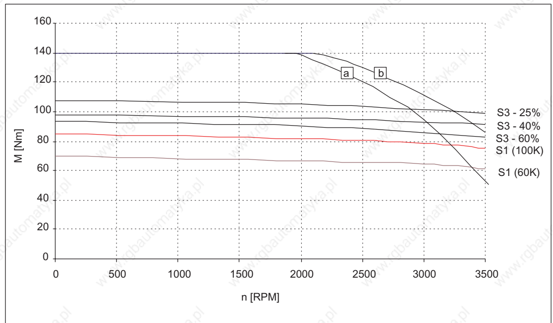
Figure 3-90 Speed-torque diagram 1FT6105-8WC7□
