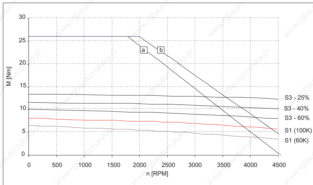
Figure 3-22 Speed-torque diagram 1FT6081-8AF7
