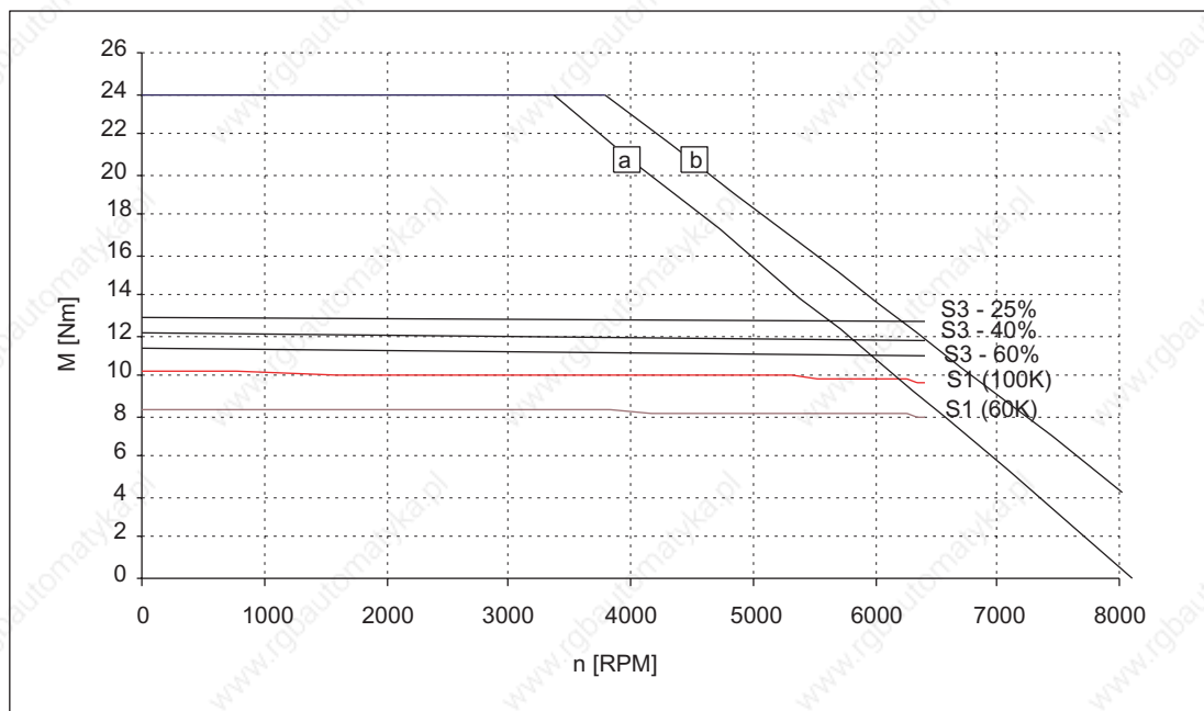
Figure 3-80 Speed-torque diagram 1FT6062-6WK7
