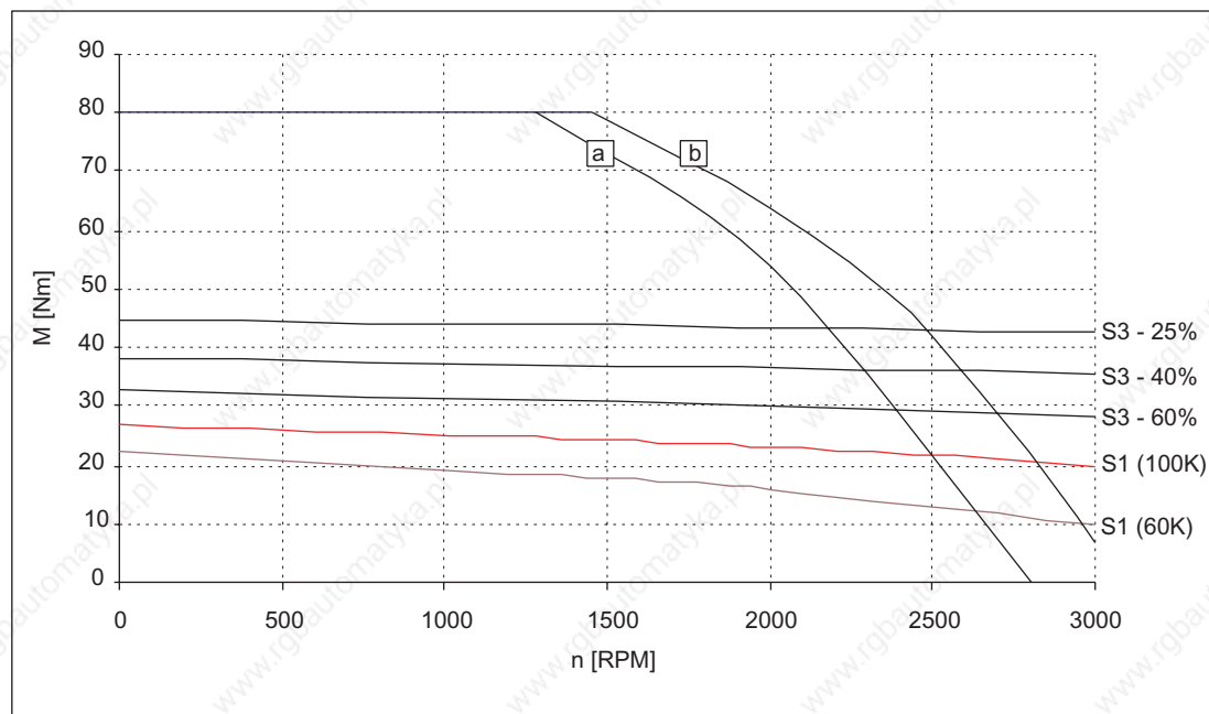
Figure 3-37 Speed-torque diagram 1FT6102-8AC7□
