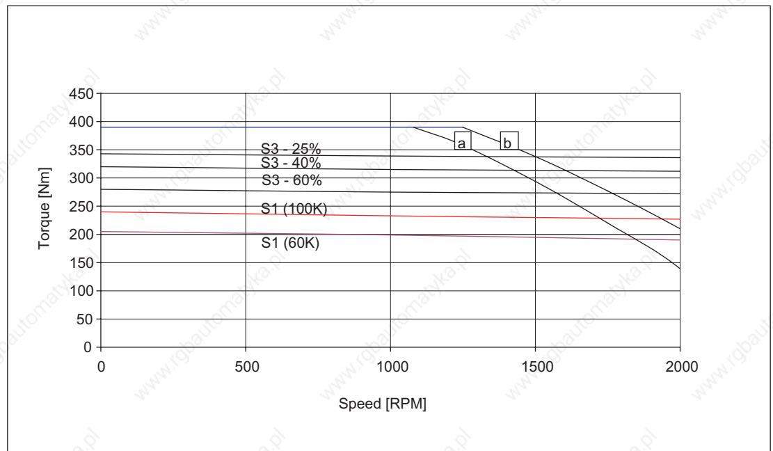
Figure 3-99 Speed-torque diagram 1FT6136-6WB7□
