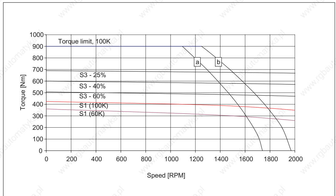
Figure 3-75 Speed-torque diagram 1FT6163-8SB7
