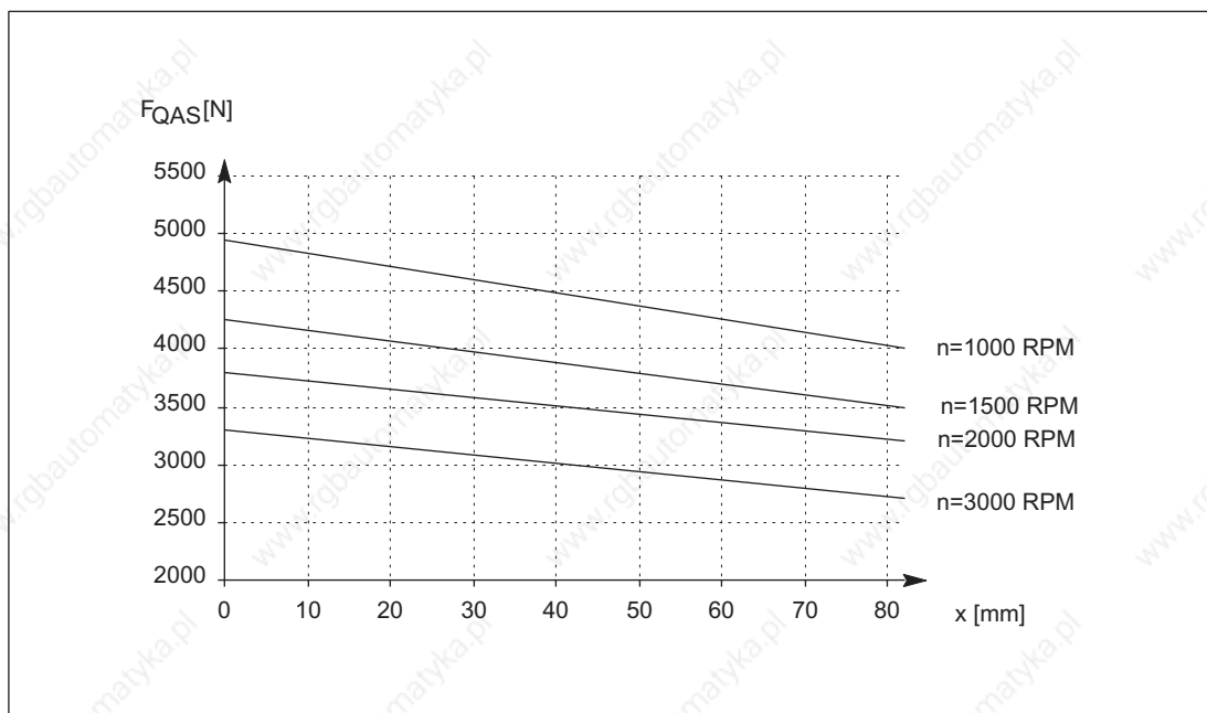
Figure 3-113 Cantilever force F_Q at a distance x from the shaft shoulder for a nominal bearing lifetime of 20,000 h
