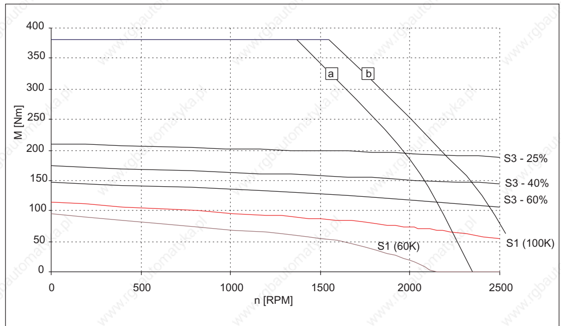
Figure 3-52 Speed-torque diagram 1FT6136-6AC71
