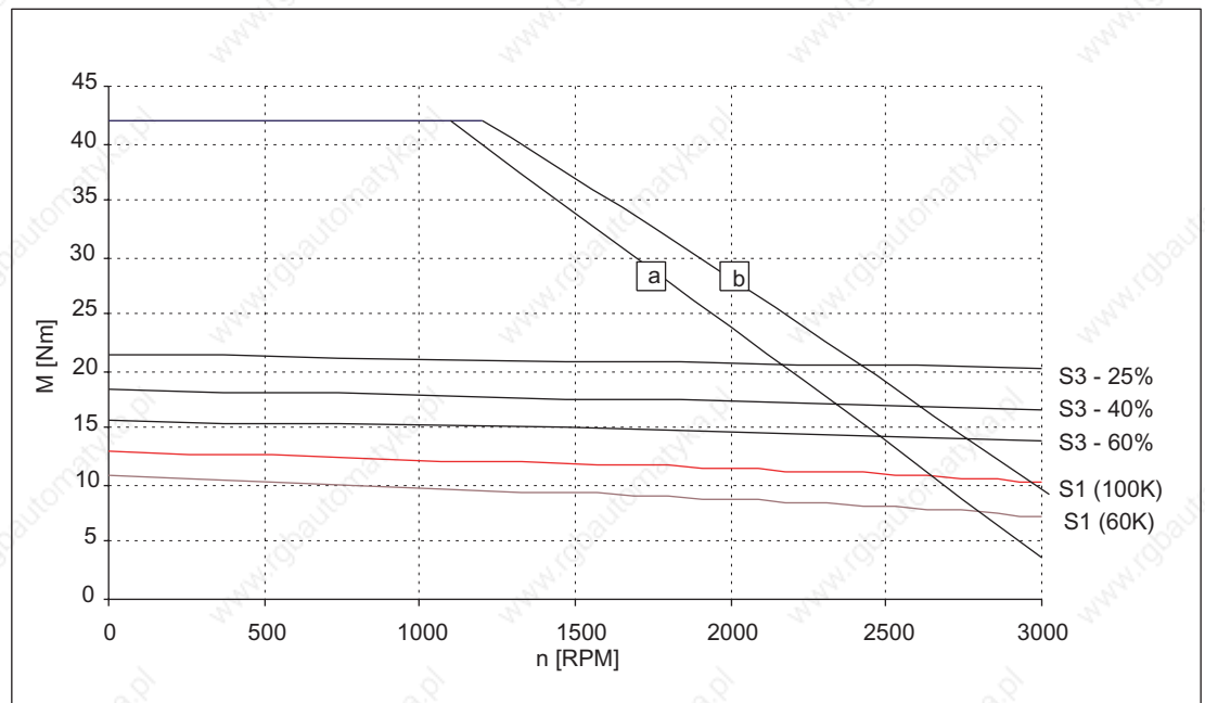
Figure 3-25 Speed-torque diagram 1FT6082-8AC7
