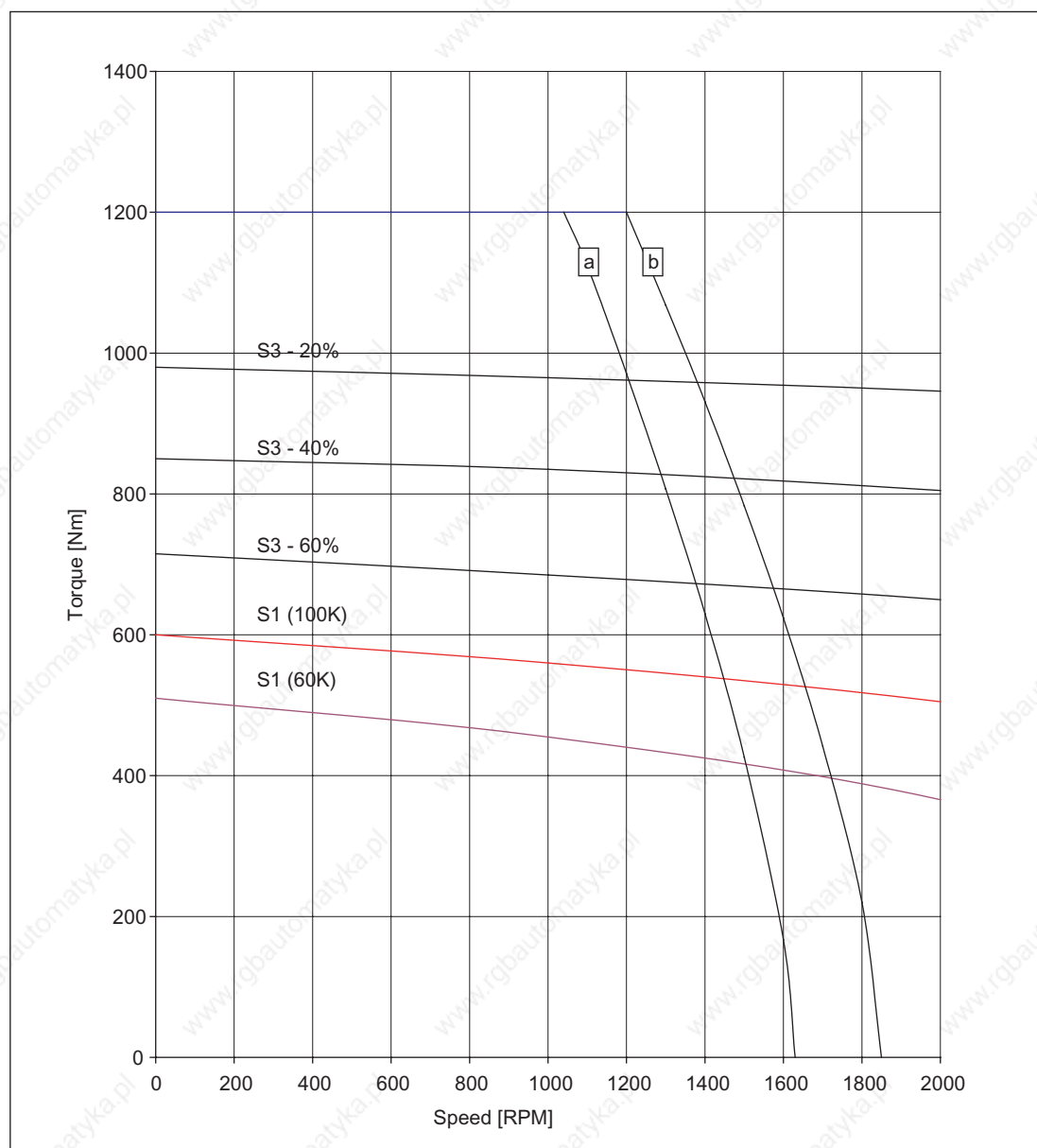
Figure 3-77 Speed-torque diagram 1FT6168-8SB7
