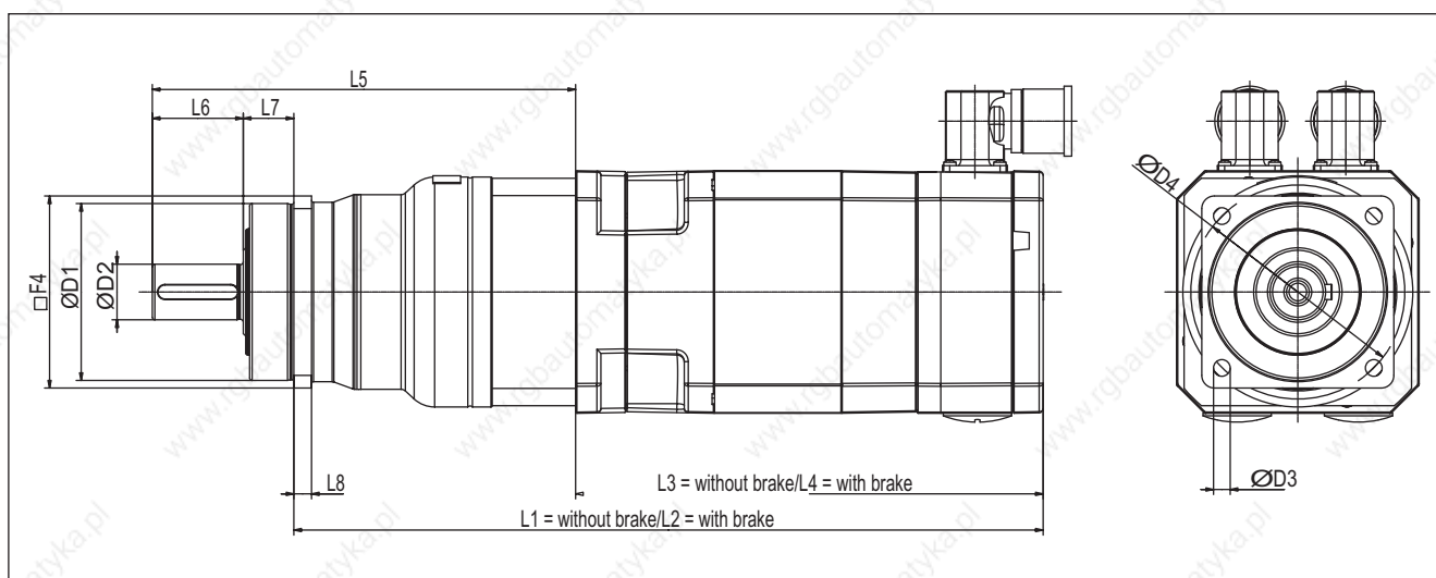
Figure 4-5 1FT6 series with 1-stage planetary gearbox (alpha company)
