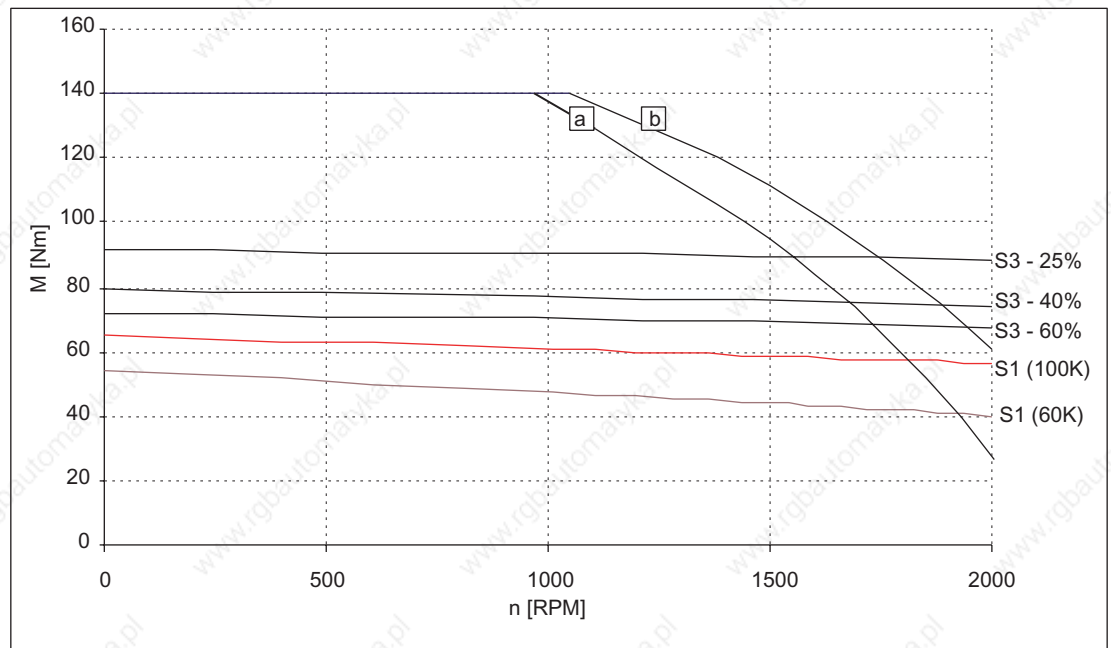
Figure 3-59 Speed-torque diagram 1FT6105-8SB7
