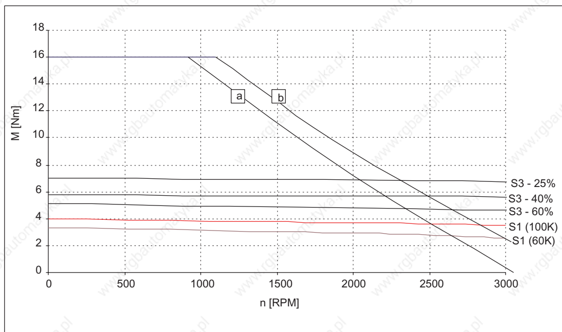
Figure 3-9 Speed-torque diagram 1FT6061-6AC7□
