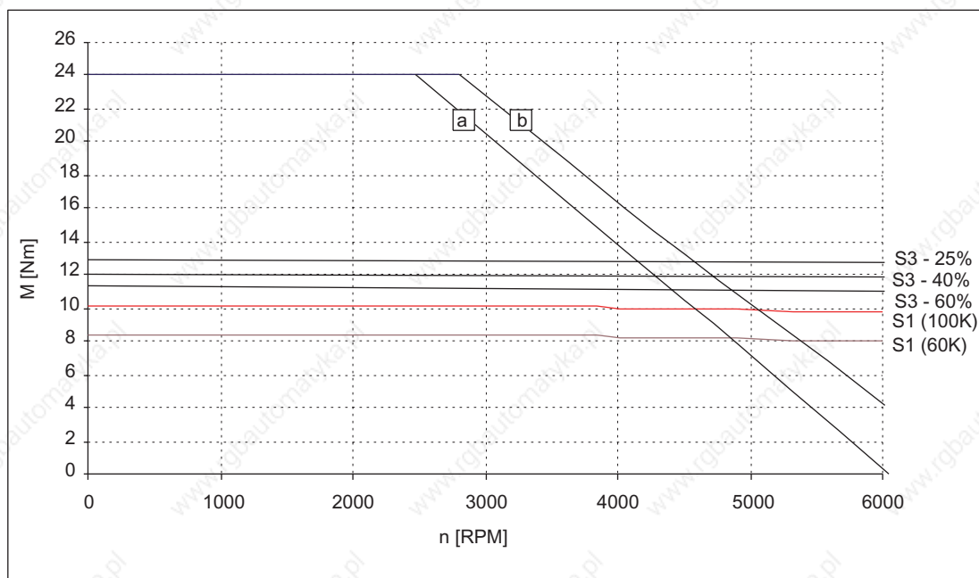
Figure 3-79 Speed-torque diagram 1FT6062-6WH7
