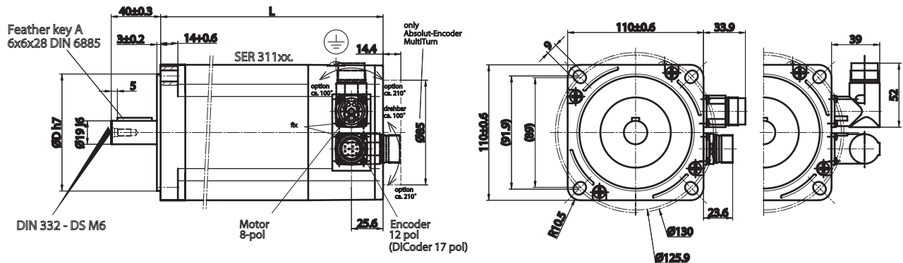
Dimensions SER311x
