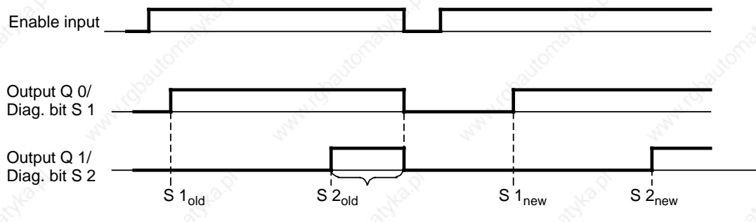
Figure 15-25. Requirement for New Setpoints
