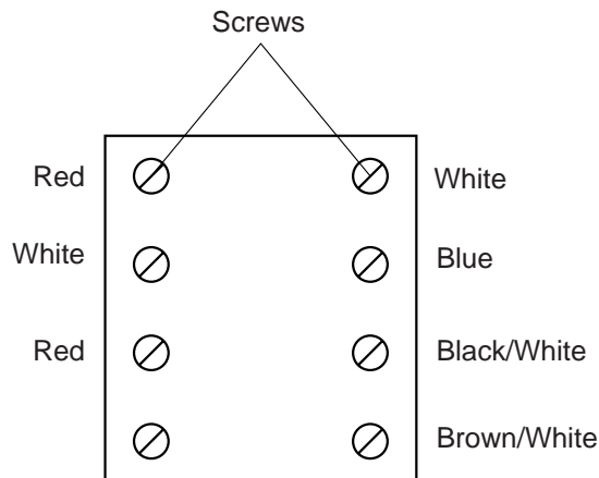
view of terminal block from above (colour of cable ends)
