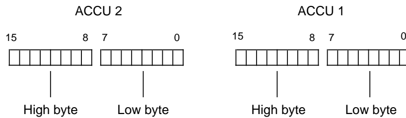
Figure 8-1. Accumulator Structure
