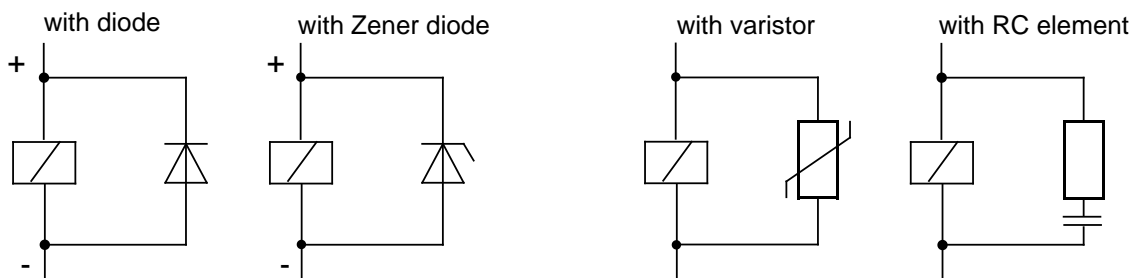
Figure 3-27. Wiring Coils
