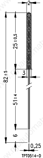
Dimensions (mm)
