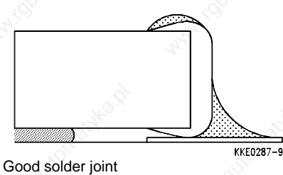
Good solder joint
