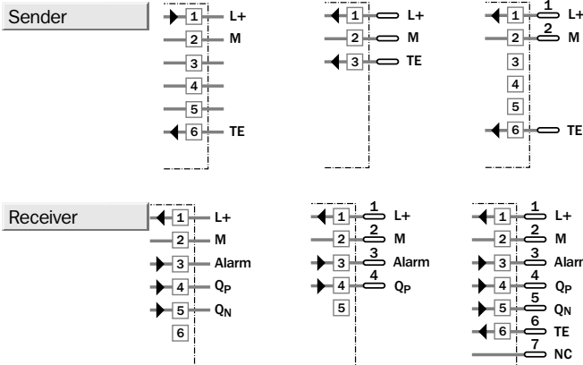
PG 11, terminals 4-pin, M 12 7-pin
