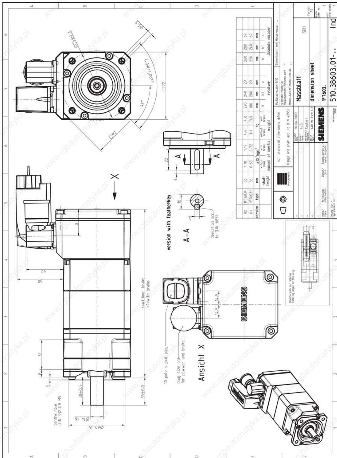
Figure 5-2 1FT603□-□A□DQ
