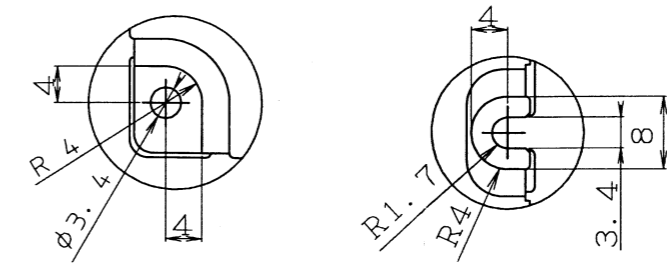
DETAIL G DETAIL H BEZEL/DISPLAY POSITION
