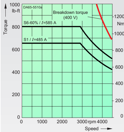
1PL6226-4.L. 1) max. breakdown torque: 1635 lb-ft/2217 Nm
