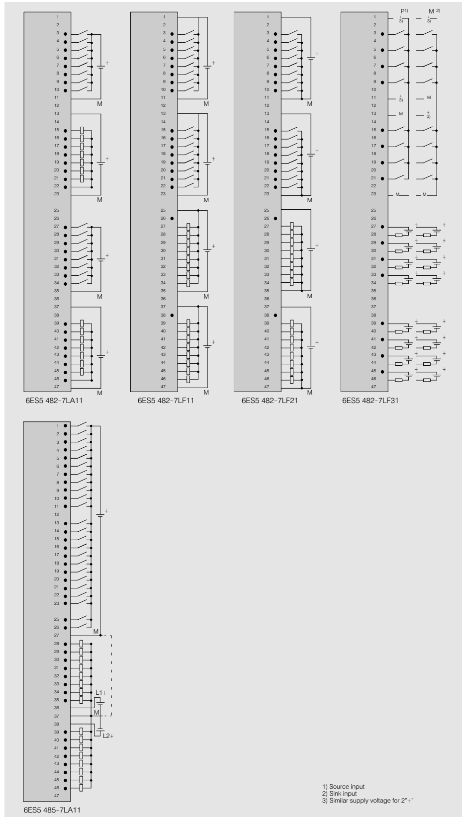
Fig. 3/29 Connection diagrams for digital input/output modules
