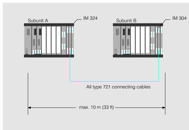
Fig. 3/40 Interfacing of central controllers
