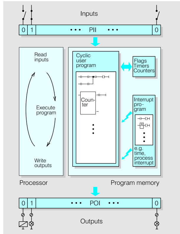
Fig. 3/4 Principle of operation of the S5-115U
