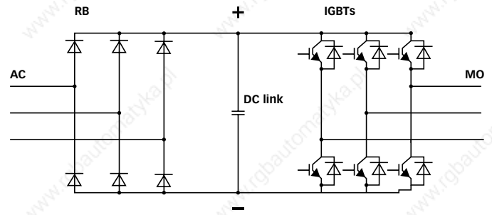
RB Rectifier bridge IGBTs Insulated gate bipolar transistors MO Motor output Rectifier bridge in a frequency converter
