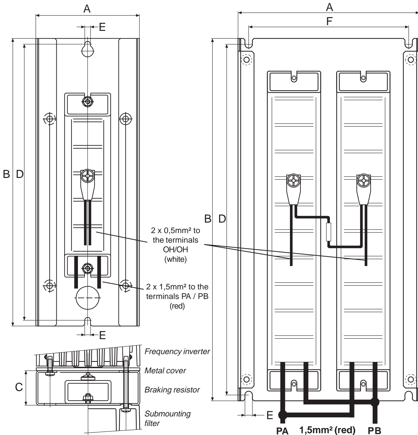
Dimensions Submounting braking resistors
