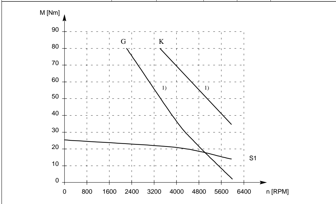
Fig. 2-21 Speed–torque diagram, 1FT5076, force ventilated
