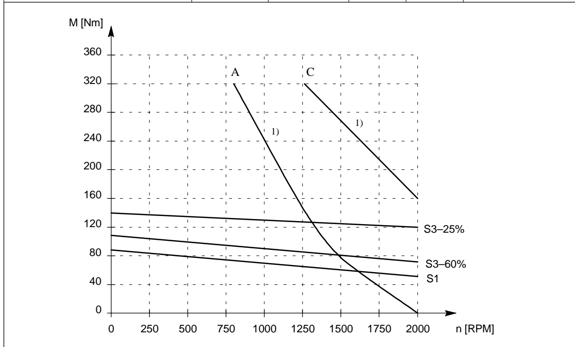
Fig. 2-17 Speed–torque diagram, 1FT5134
