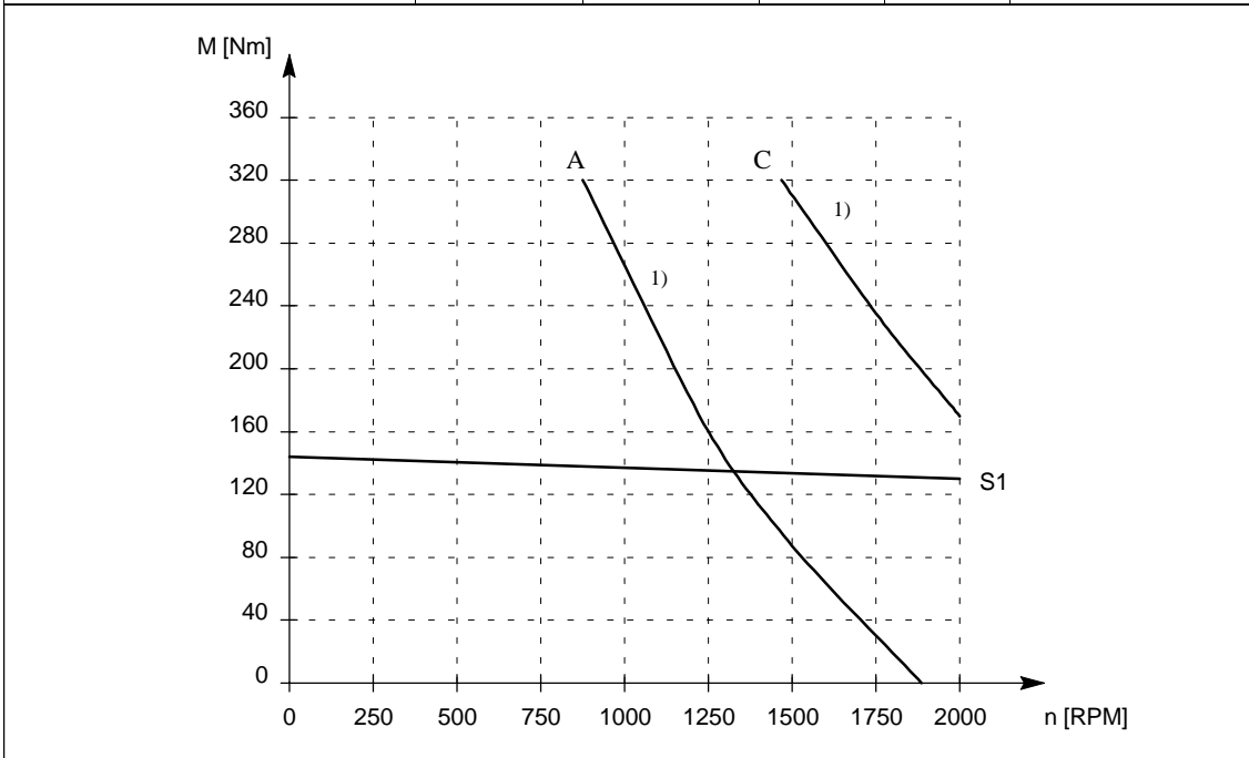
Fig. 2-27 Speed–torque diagram, 1FT5136, force ventilated
