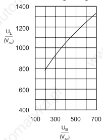
Arc voltage-Diagram
