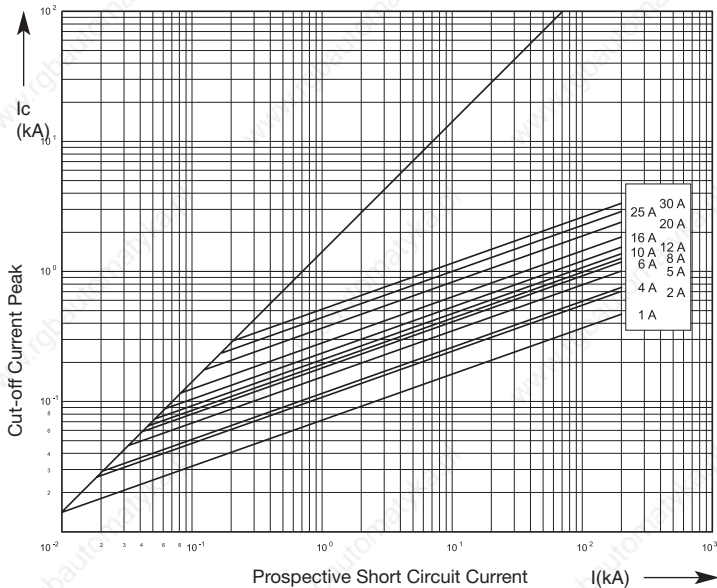
Cut-Off Characteristics
