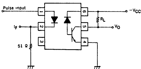
** Measuring circuit
