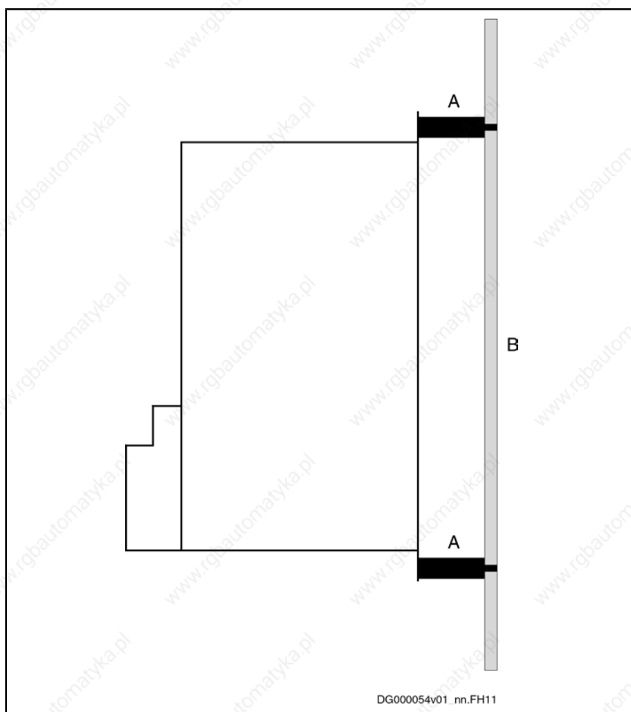
Fig. 14-56: How to use the control cabinet adapters
