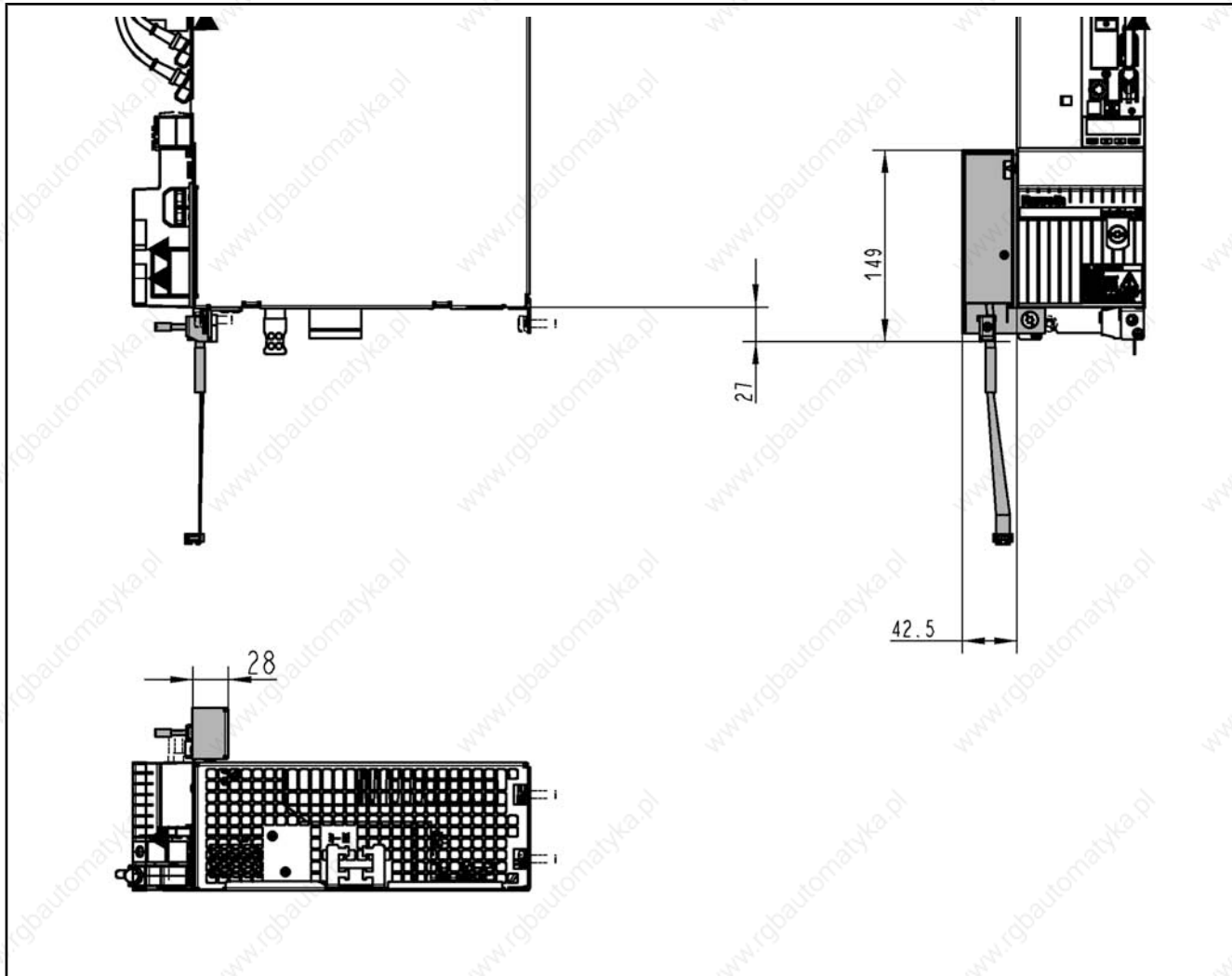
Fig.14-139: Dimensions RKB0001
