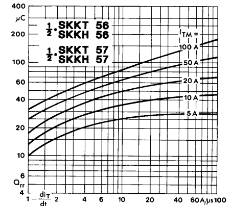
Fig. 5 Recovered charge vs. current decrease
