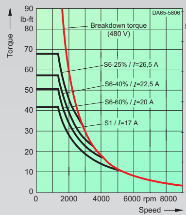
1PH7107-2.D.-..... max. breakdown torque: 100 lb-ft/135 Nm
