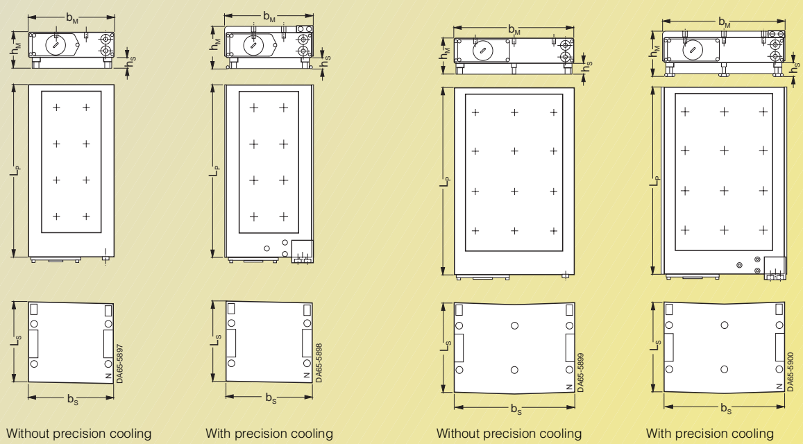
Without precision cooling With precision cooling Sizes 1FN3 050 through 1FN3 450
