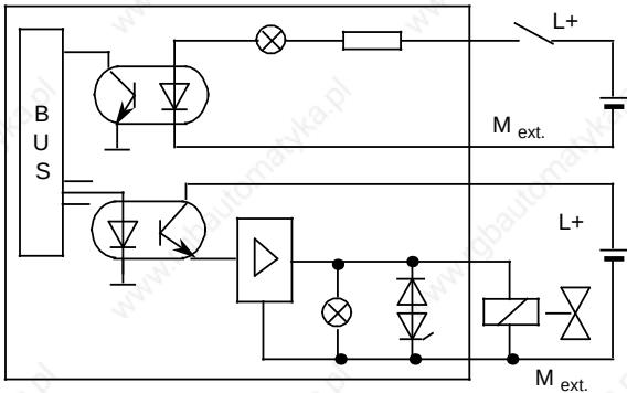
Block diagram
