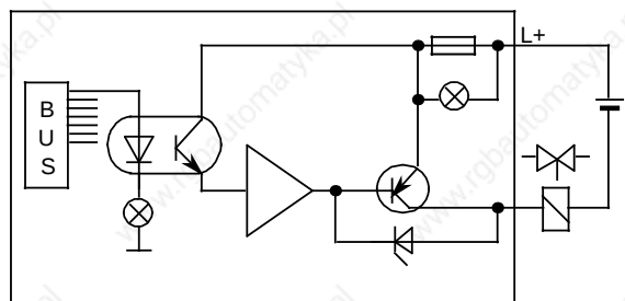
Block diagram
