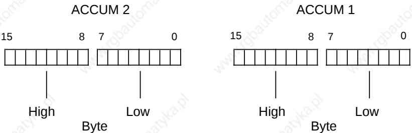
Figure 8-1. Accumulator Structure
