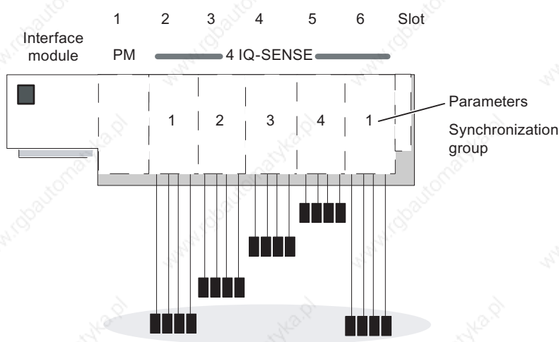
Figure 5-1 Synchronization group
