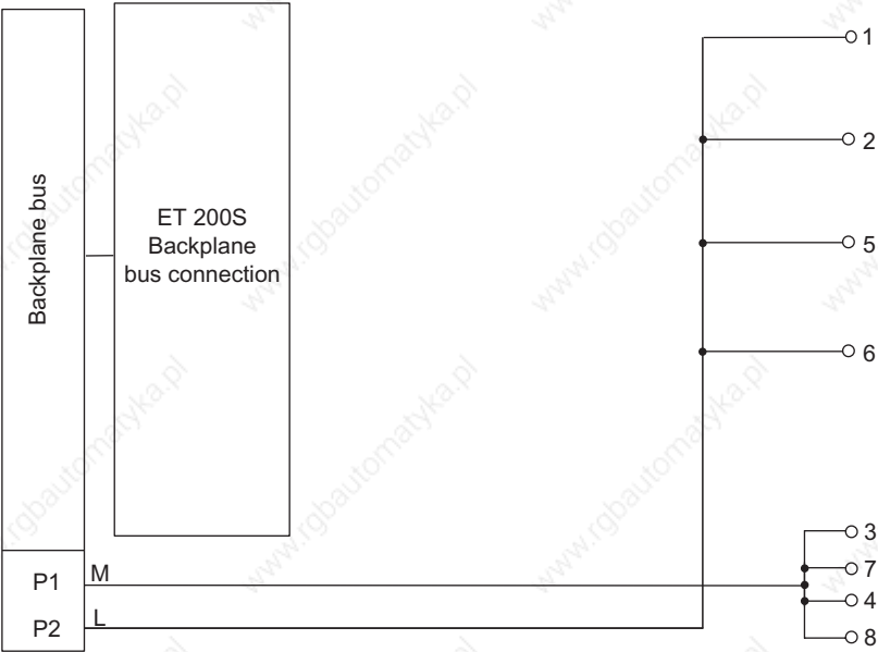
Figure 6-1 Block diagram of the 4POTDIS
