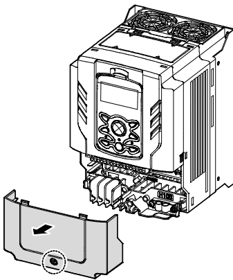
Modele 0.75–30 kW
