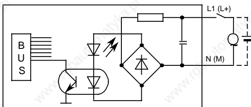
Block diagram
