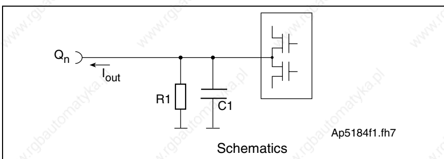
Fig. 6-30: Output circuit
