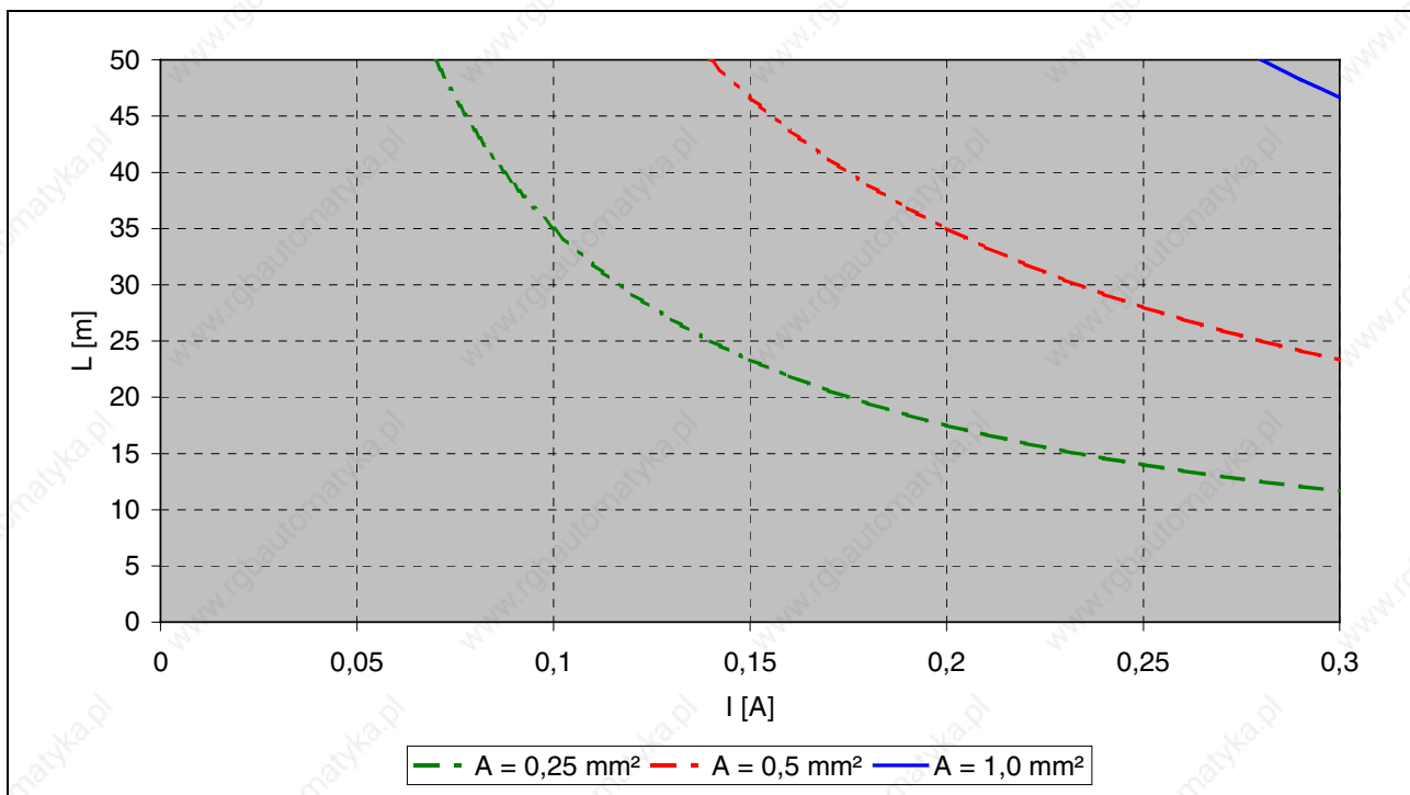
Fig. 4-120: With sensor connection
