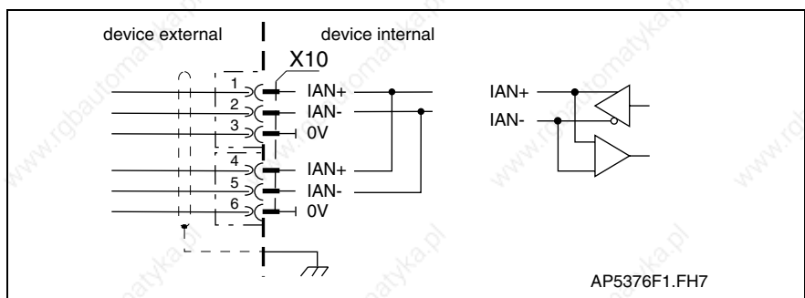
Fig. 4-136: Expansion interface
