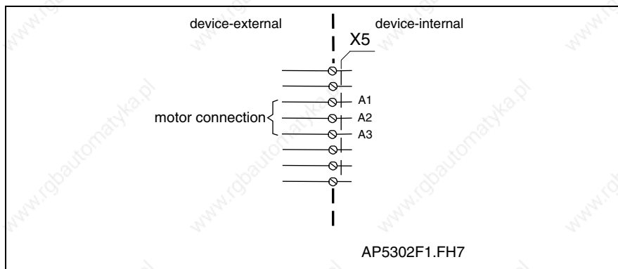
Fig. 4-94: Motor connections
