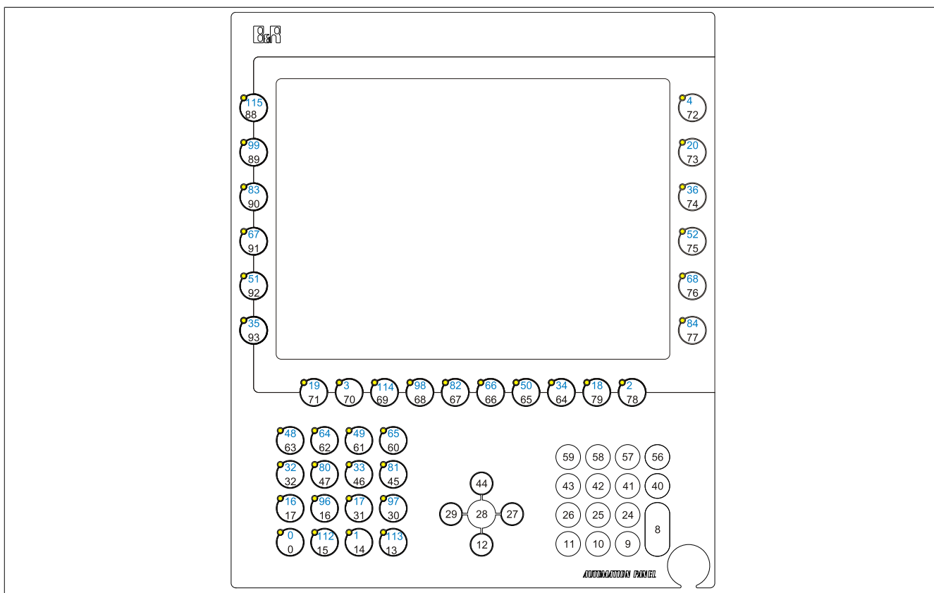
Figure 103: 5AP951.1043-01 / 5AP981.1043-01 - Hardware numbers
