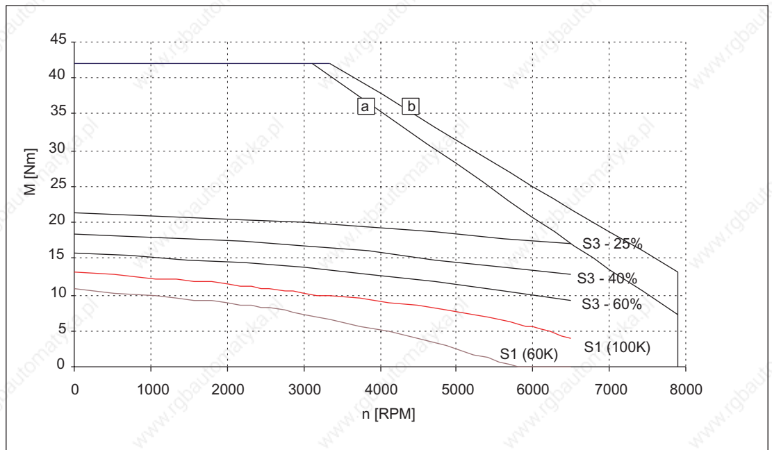
Figure 3-28 Speed-torque diagram 1FT6082-8AK7□
