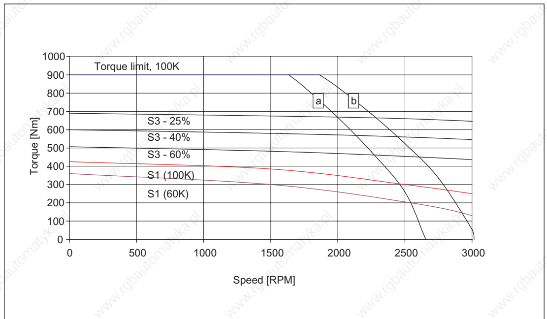
Figure 3-76 Speed-torque diagram 1FT6163-8SD7
