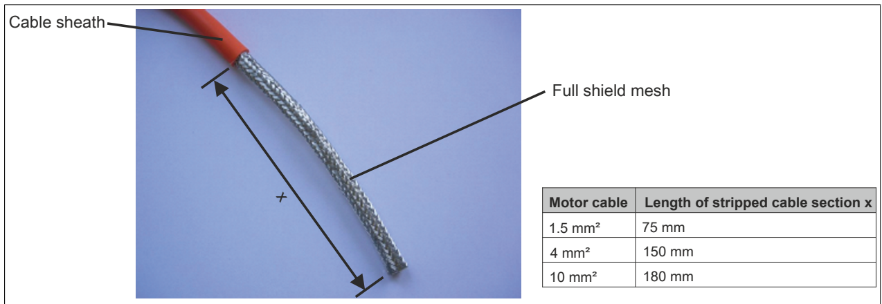
Figure 68: Stripped cable end
