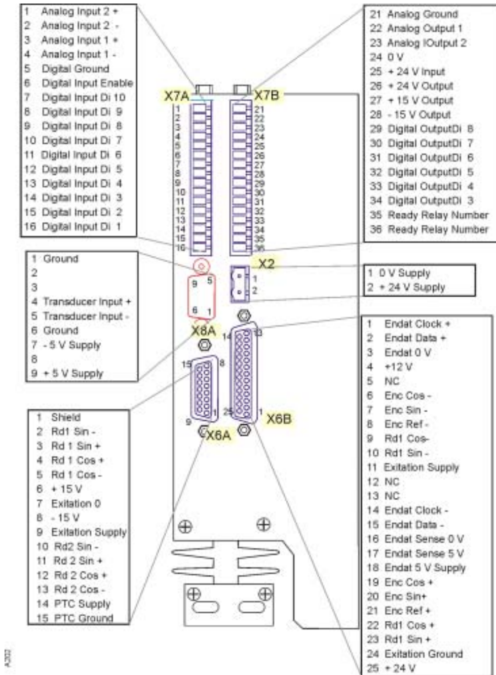
Figure 17. I/O Connections for all DMC 2 units, bottom view.
