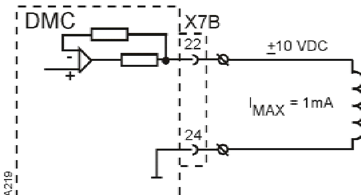
Figure 28. Analog output.
