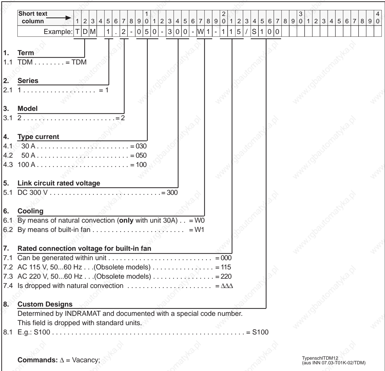
Figure 113: Type codes for servo-drive module TDM
