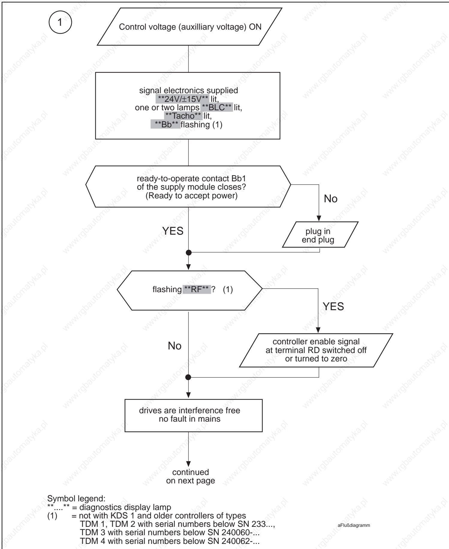
Figure 72: Power-Up Sequence
