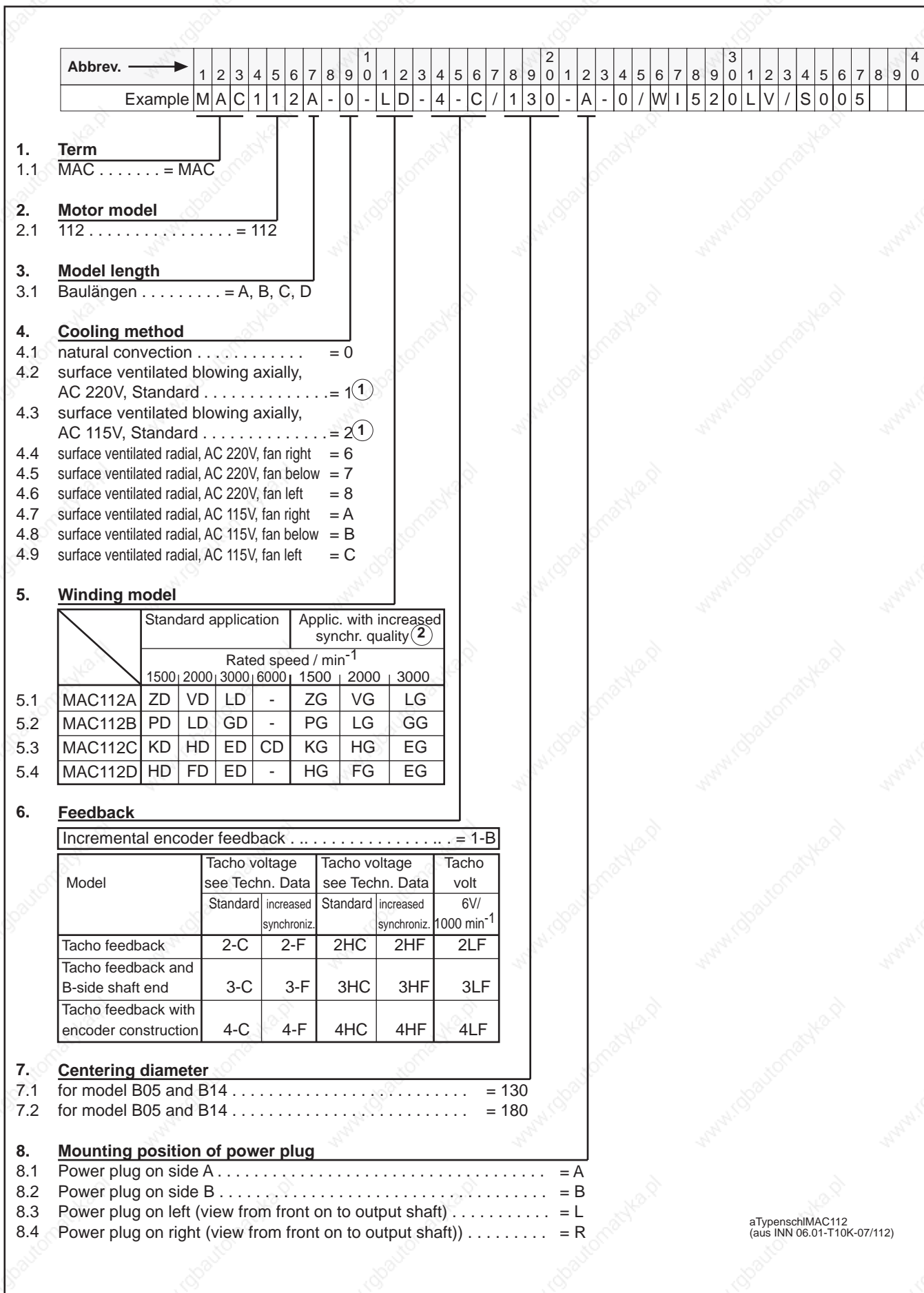
Figure 112: Type Key for MAC Servo-Motor
