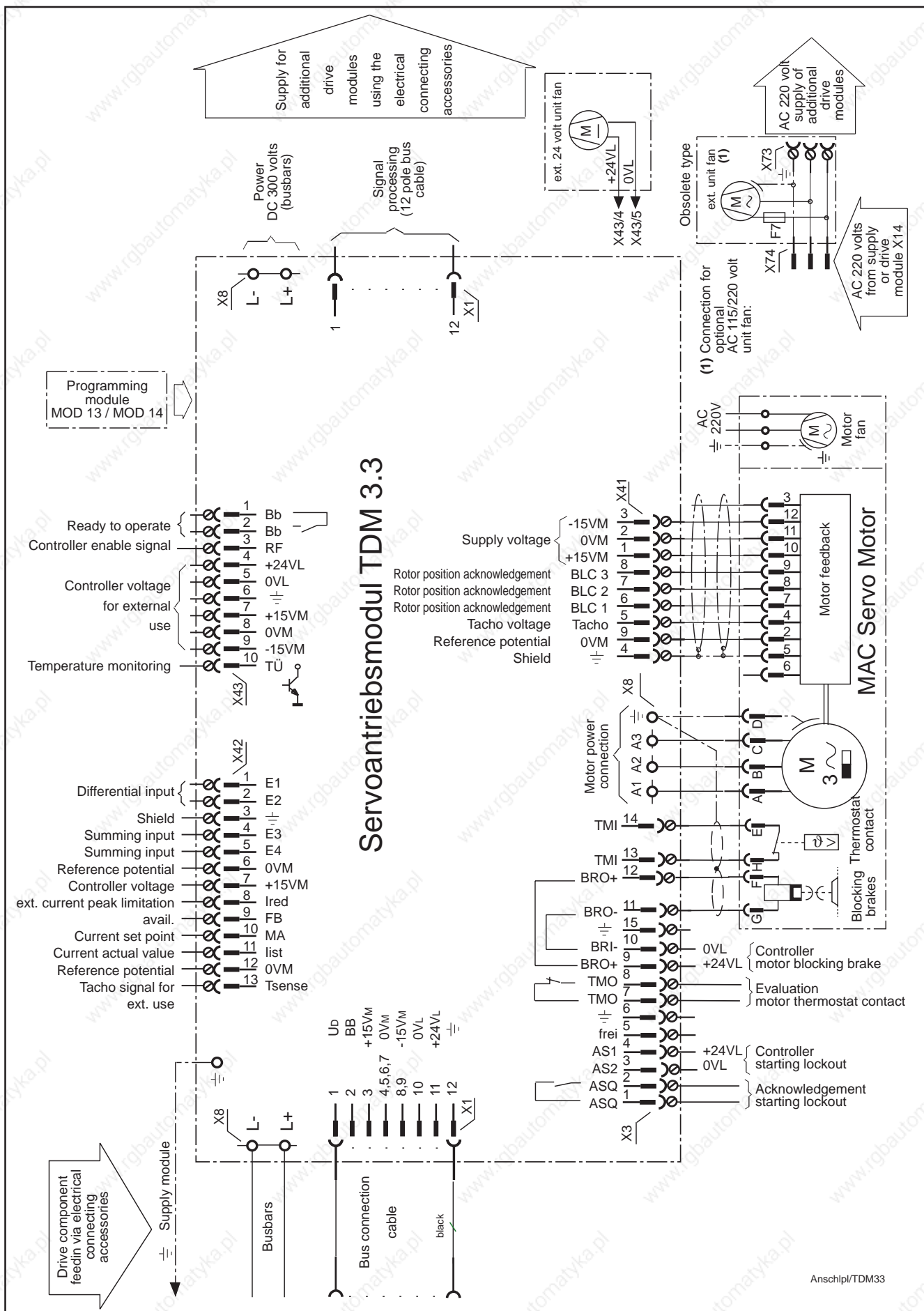
Figure 17: Connection plan for TDM 3.3
