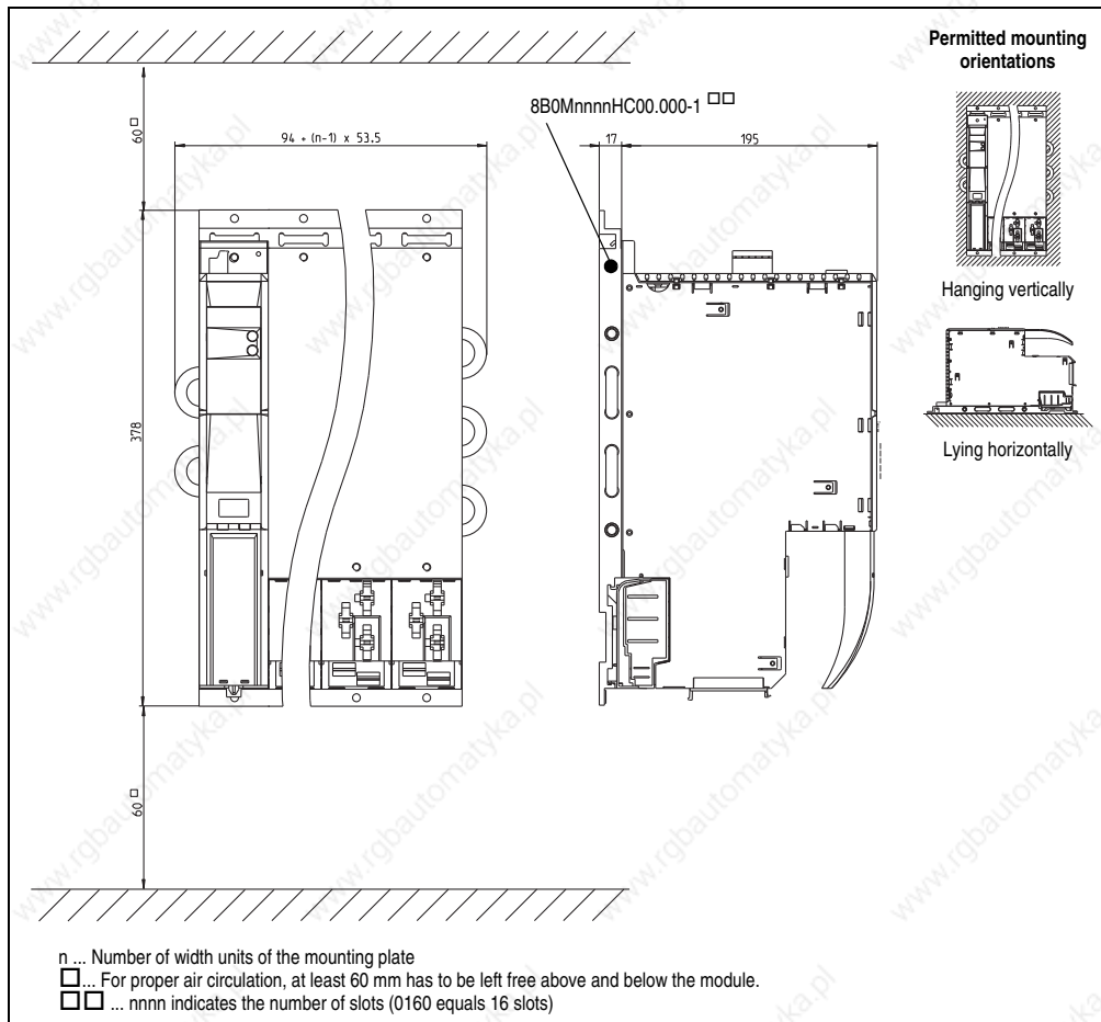
Figure 54: Dimensional diagram and installation dimensions for 8B0C0160HC00.000-1, 8B0C0320HC00.000-1
