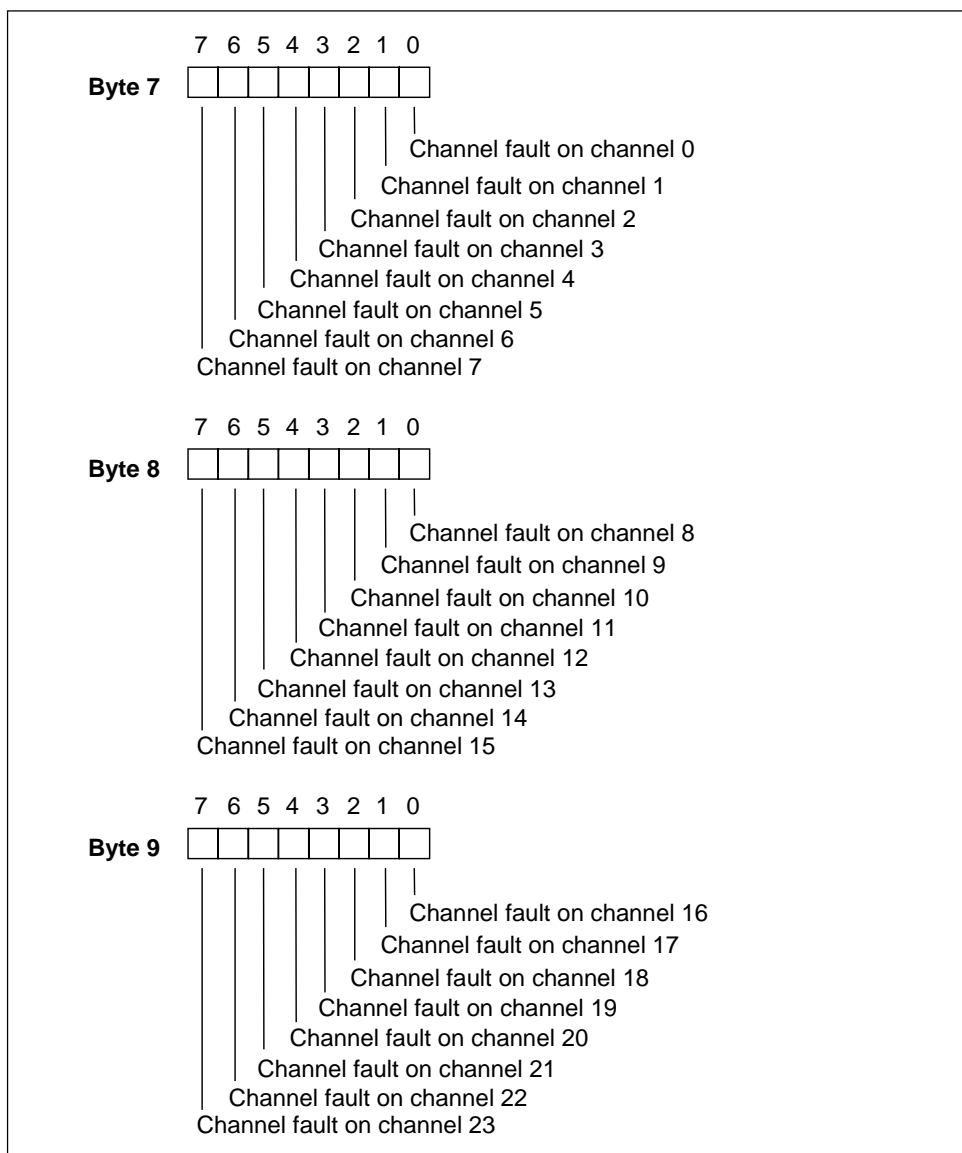
Figure A-4 Bytes 7 to 9 of the Diagnostic Data for the SM 326; DI 24 × 24V DC; with Diagnostic Interrupt
