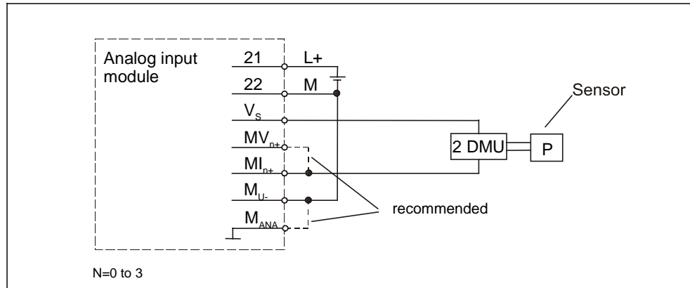
Figure 5-8 Improvement of Accuracy in the Case of Current Measurement on Channels 0 to 3 with 2 WMT
