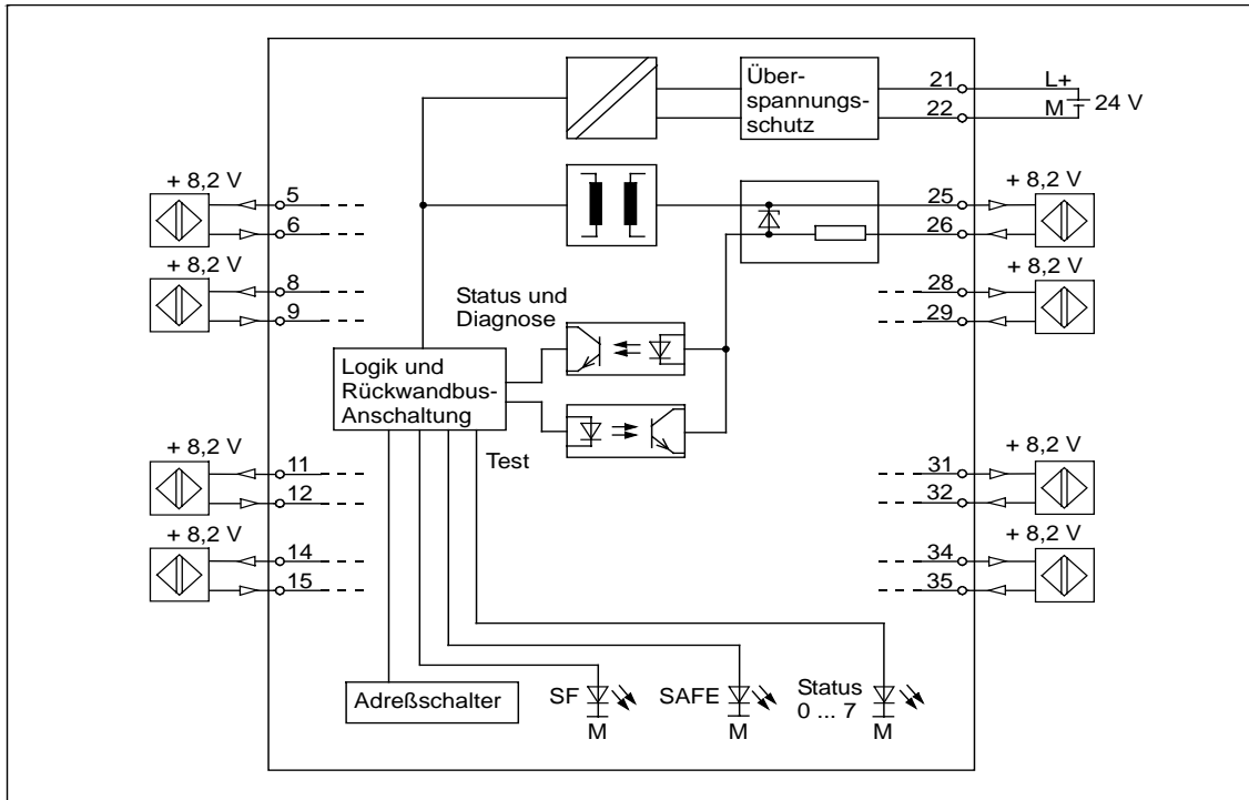
Figure 9-20 Terminal Assignment and Block Diagram of the SM 326; DI 8 X NAMUR; with Diagnostic Interrupt
