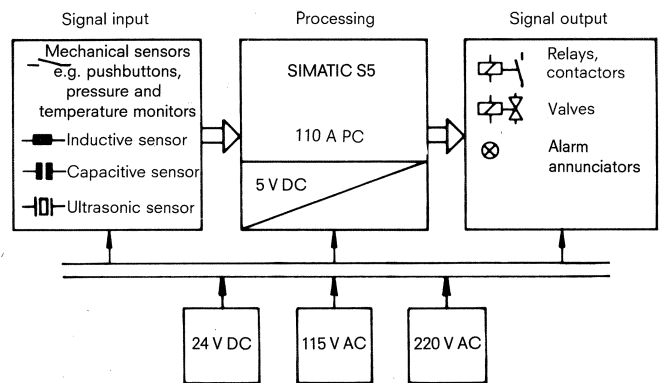
Fig. 2 Structure of a system using the S5-110A programmable controller
