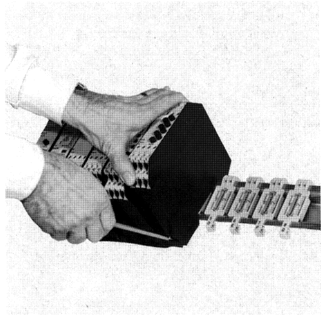
Fig. 17 Removing an I/O module
