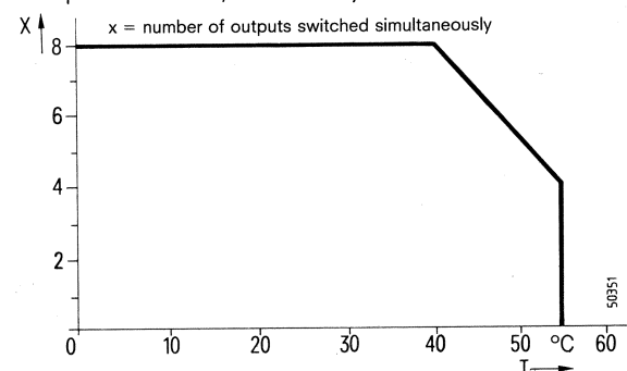
Permissible number of simultaneously switched outputs as a function of ambient temperature.
