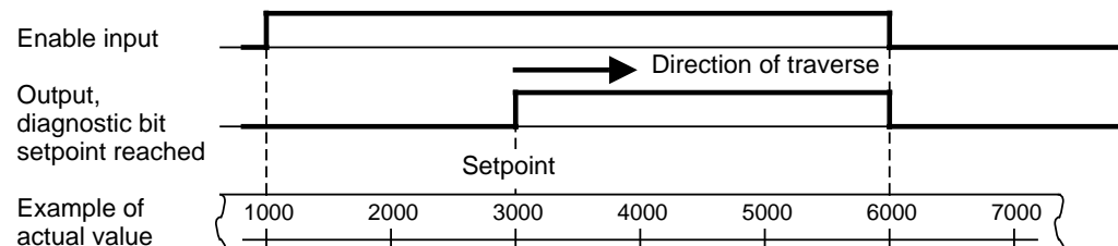
Figure 15-22. Approaching a Setpoint in Up-Count Direction
