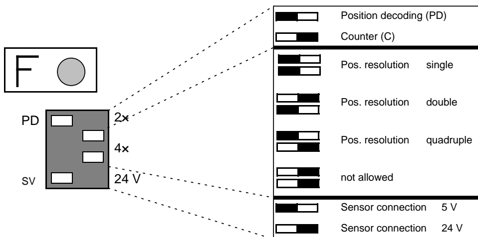
Figure 15-7. Switch Positions on the Operating Mode Switch
