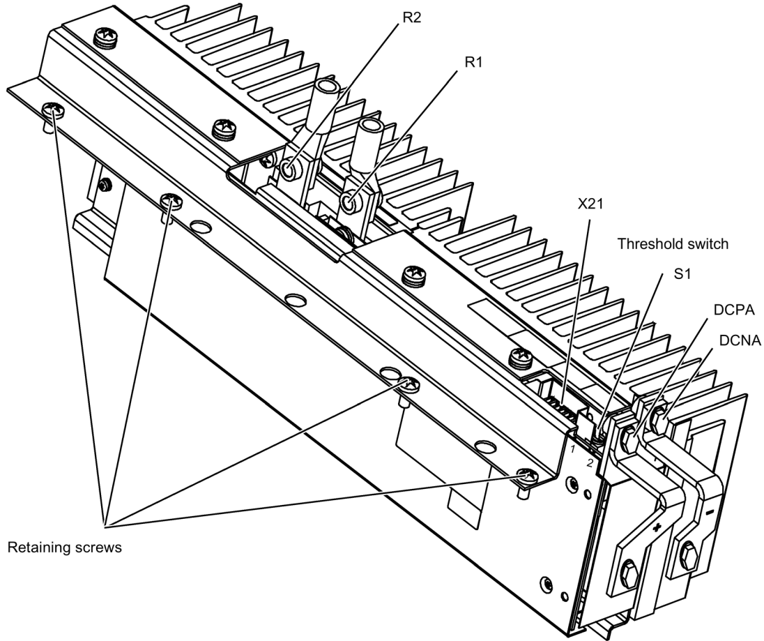
Figure 7-4 Braking Module for Smart Line Module / Active Line Module / Motor Module, frame sizes HX / JX
