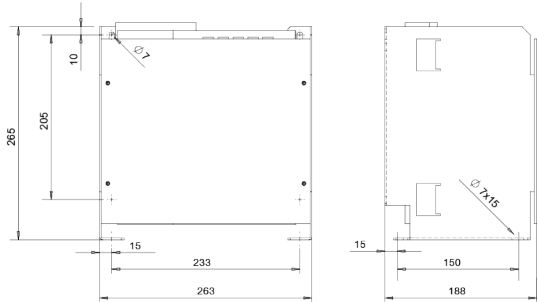
Figure 8-11 Dimension drawing of the voltage peak limiter, type 1
