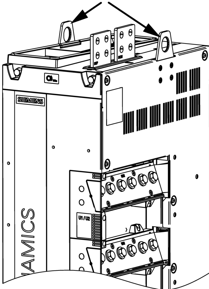
Figure 10-5 Crane lifting lugs for Motor Module Chassis-2, frame size FS4
